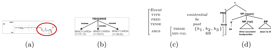
Figure 1: Tasks in NLG, illustrated with a simplified example from the neonatal intensive care domain. First the system has to decide what the important events are in the data (a, content determination), in this case, occurrences of low heart rate (bradycardias). Then it has to decide in which order it wants to present data to the reader (b, text structuring) and how to express these in individual sentence plans (c, aggregation, lexicalisation, reference). Finally, the resulting sentences are generated (d, linguistic realisation).
