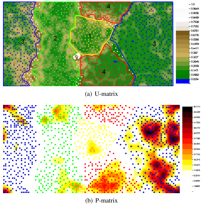
Fig. 5. Visualization maps of the highest-performing ESOM obtained and the 4 clusters identified. The 1365 best-matching neurons are drawn as squares on top of the maps. The maps illustrated are border-less since the map grid is organized in a toroid shape.
