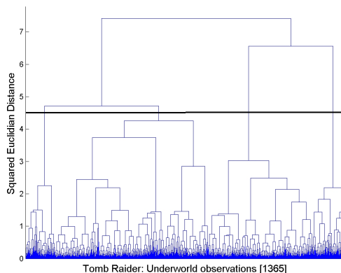
Fig. 3. Clustering of data using the Ward dendrogram method. A T value of 4.5 (illustrated with a horizontal black line) reveals 4 clusters.
