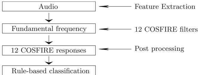
Fig. 3. The main steps of our proposed method. The audio signal is converted in to its fundamental frequency (pitch track). 12 COSFIRE filters are configured using the frequencies of the 12 western notes. The COSFIRE filters are applied to the pitch track, returning 12 responses, one for each COSFIRE filter. The responses are then binarized and post processed. Rule-based approach is used to identify and classify ornamentations.
