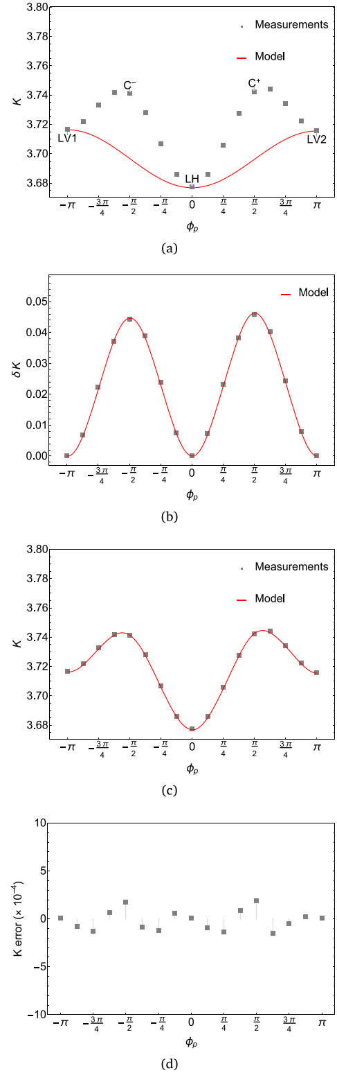
Fig. 11. The fitting procedures and performance of the example at minimum gap R = 3.25 mm: (a) With the fitting model using the Eq. (13), the asymmetry between the transition from LH to LV is subtracted. (b) After the subtraction, we fit the residual part using the model of Eq. (17). (c) Combining the models in (a) and (b), we obtain the final model for the measurements. (d) Relative error of the model in (c), compared with measurements data.
