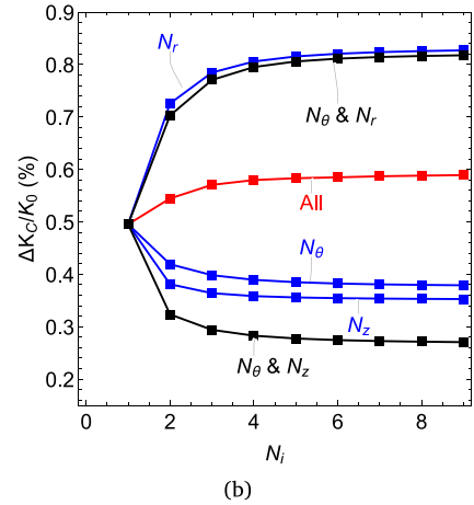
Fig. 4. (a) 3D schema of an example with subdivision \{3, 8, 2\} . (b) In the case of zebra -type structure with mixed material \text{SmCo}_5 (axial) and \text{Sm}_2\text{Co}_{17} (radial) at R = 3.25 mm, the relative \Delta K_C (see Eq. (3)) compared with K_0 ( K_{LH} at minimum gap radius) versus subdivisions. Cylindrical geometry and shaped field simulation were applied. (For interpretation of the references to colour in this figure legend, the reader is referred to the web version of this article.)
