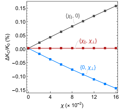
(b) Single material Halbach structure
