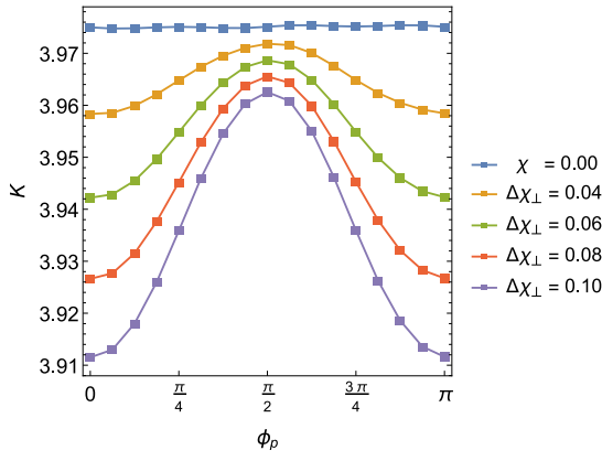
Fig. 9. The deflection parameter K as a function of the phase shift in parallel operational mode for a series of \Delta\chi_{\perp} in zebra structure, where \Delta\chi is the difference between the \chi of radial magnets with respect to axial magnets.
