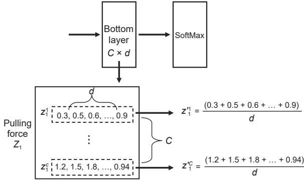
Fig. 2 The computation of Z_i^j . The figure shows a toy example of Z_1^j formation. The bottom layer is shaped as C \times d , thus pulling force Z_1 has the same shape. Z_1 has C vectors as z_i^j , which contains d values. For every z_i^j , we average it to get Z_i^j .
