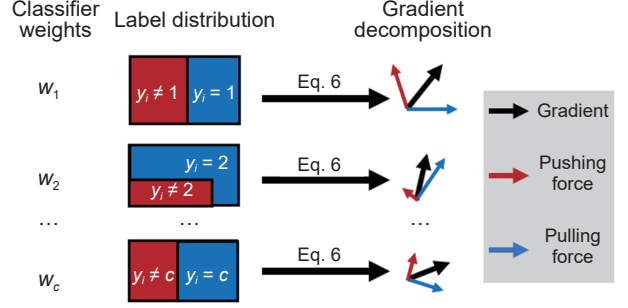
Fig. 1 Classifier Weights Gradient Composition. In a c -th classes classification task, the gradient of each weight in the classifier can be divided into pulling force and pushing force by data labeled as c and labeled not as c .
