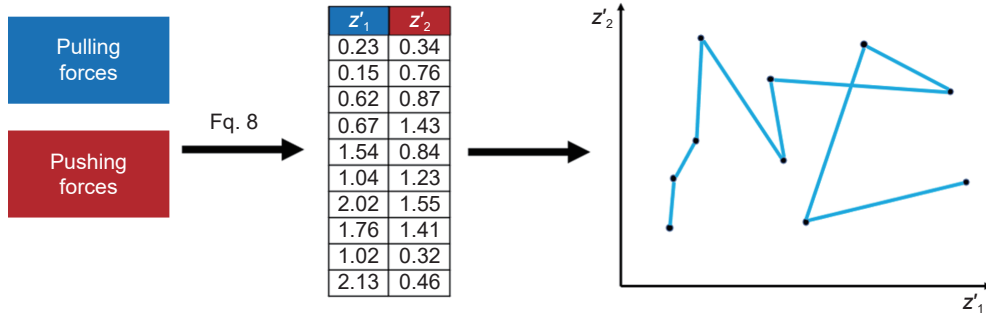
Fig. 3 The formation of gradient trajectory. In a 10-th classes classification task, a client calculates its pulling force and pushing force, gets Z'_1 and Z'_2 , and plots the trajectory in a two-dimensional space, where x-axis is for Z'_1 and y-axis is for Z'_2 .
