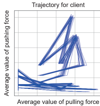
Fig. 5 Gradient Trajectories of 100 clients in an FL System. The trajectories of the 100 clients form several distributions, showing a clear trend of clustering.
