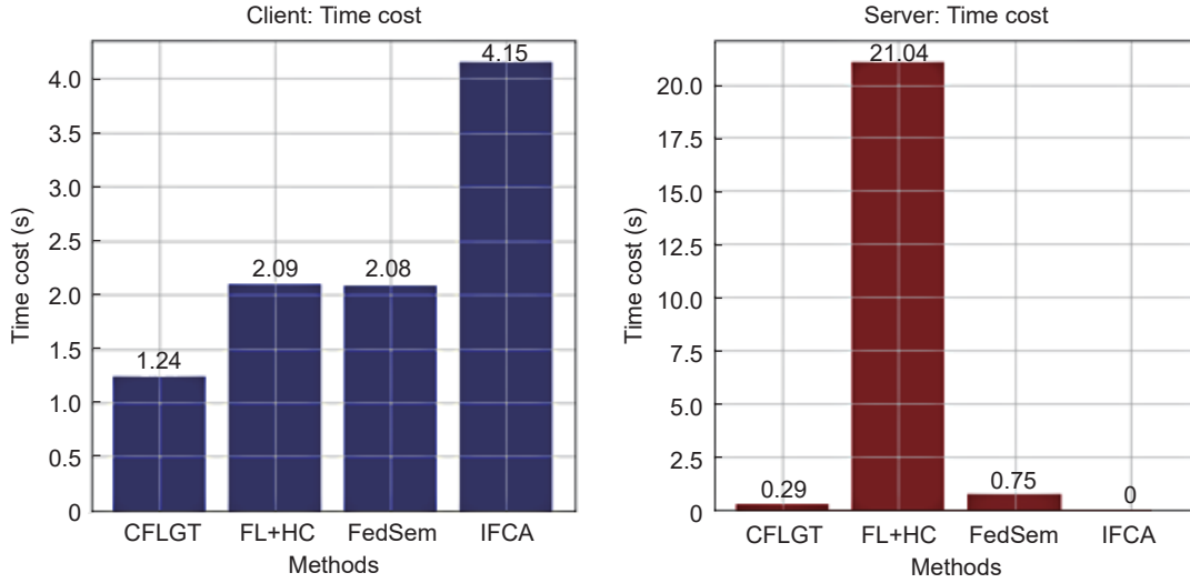
Fig. 8 Efficiency Comparison. The left result represents the time cost of the client. The right result represents the time cost of the server.
