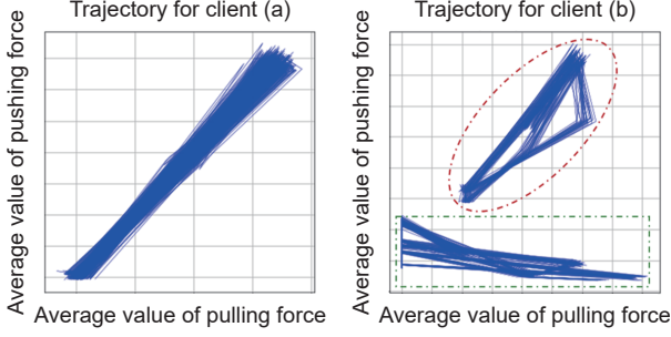
Fig. 4 Gradient Trajectories of all Clients in an FL System. The trajectories in (a) are from IID data and trajectories in (b) are from heterogeneous data.
