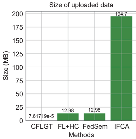
Fig. 9 Efficiency Comparison. The result represents the size of uploaded data from client to server.
