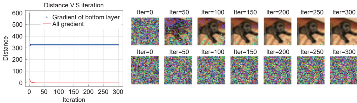
Fig. 10 Results in Gradient Leakage. The two sets of images on the right display the update of the fake image to the original image as iteration grows. The upper one is based on the gradient of the whole model and another one is based on the gradient of the bottom layer of the model. The figure on the left shows the change in gradient distance as the iteration increases.
