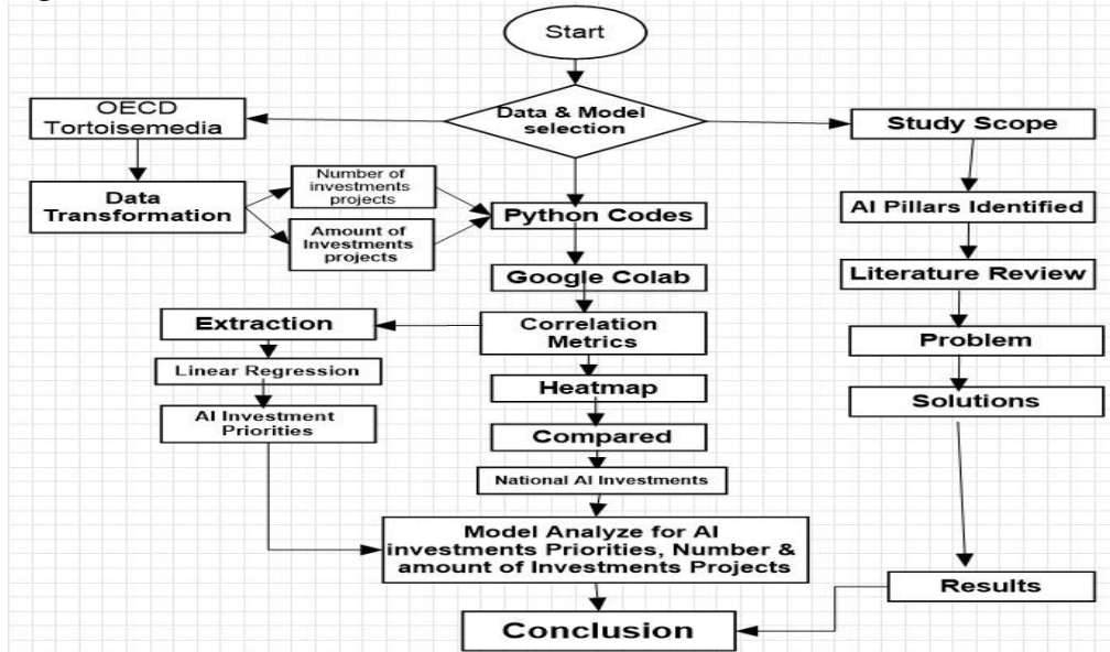
Figure 8. Method Flowchart
