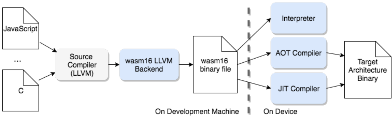
Figure 1. wasm16 compiler and execution toolchain.
