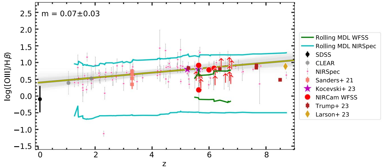
Figure 5. The \log[\text{O III}]/\text{H}\beta emission-line ratio vs. redshift. The black point is the median redshift and \log[\text{O III}]/\text{H}\beta of the SDSS sample (York et al. 2000), with the error bars representing the standard deviation of the sample. The gray points and pink squares are from the CLEAR and MOSDEF samples, respectively (Sanders et al. 2021; Simons et al. 2023). The SMACS observations are marked as crimson squares. NIRSpect AGN from CEERS are purple stars. The NIRSpect and WFSS samples are represented by pink points and red points and arrows, respectively. The yellow line is the linear fit to the NIRSpect. The cyan lines represent the rolling median detection limit (MDL) to the best-fit line for the NIRSpect galaxies, indicating the range of galaxies we could see based on our S/N cutoffs. This increase of [\text{O III}]/\text{H}\beta with redshift is also shown in the linear fit line, with a slope of (0.06 \pm 0.02) .
