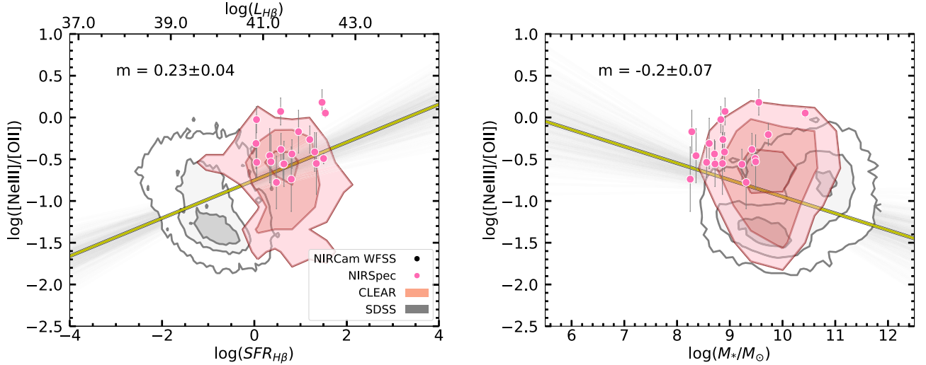
Figure 9. Left: The relationships between the [\text{Ne III}]/[\text{O II}] emission-line ratio and the galaxy \text{H}\beta luminosity and \text{H}\beta SFR. Right: The relationships between the [\text{Ne III}]/[\text{O II}] emission-line ratio and stellar mass. In both panels, the gray and red contours are the SDSS and CLEAR sample, respectively. The black points and arrows are [\text{O III}]/\text{H}\beta measurements and limits from NIRCам WFSS observations. The yellow line is fit to the CEERS z > 5 sample and randomly selected SDSS and CLEAR galaxies matching the size of the CEERS sample. There is a significant ( >3\sigma ) relationship between [\text{Ne III}]/[\text{O II}] and \text{H}\beta SFR, and a marginal relationship ( 2.8\sigma ) with stellar mass.
