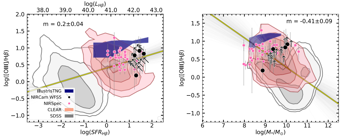
Figure 8. Left: The relationships between the [\text{O III}]/\text{H}\beta emission-line ratio and the galaxy \text{H}\beta luminosity and \text{H}\beta SFR. Right: The relationships between the [\text{O III}]/\text{H}\beta emission-line ratio and stellar mass. In both panels, the gray and red contours are the SDSS and CLEAR samples, respectively. The black points and arrows are [\text{O III}]/\text{H}\beta measurements and limits from NIRCам WFSS observations. The yellow line is fit to the CEERS z > 5 sample and randomly selected SDSS and CLEAR galaxies matching the size of the CEERS sample. All the IllustrisTNG simulations are shown as the purple region.
