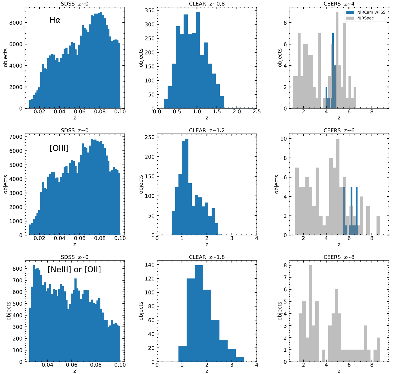
Figure 2. Distribution of redshifts for each emission-line sample: H\alpha (top), [O III] (middle), and [Ne III] and [O II] (bottom). These are named by their respective emission lines, which have S/N > 3 ; in the case of [Ne III] and [O II] , either line may reach this requirement. The samples come from the SDSS(left), CLEAR (middle), and CEERS(right). In the right panel, the gray histograms are the NIRSpec observations and the blue ones are NIRCcam WFSS.
