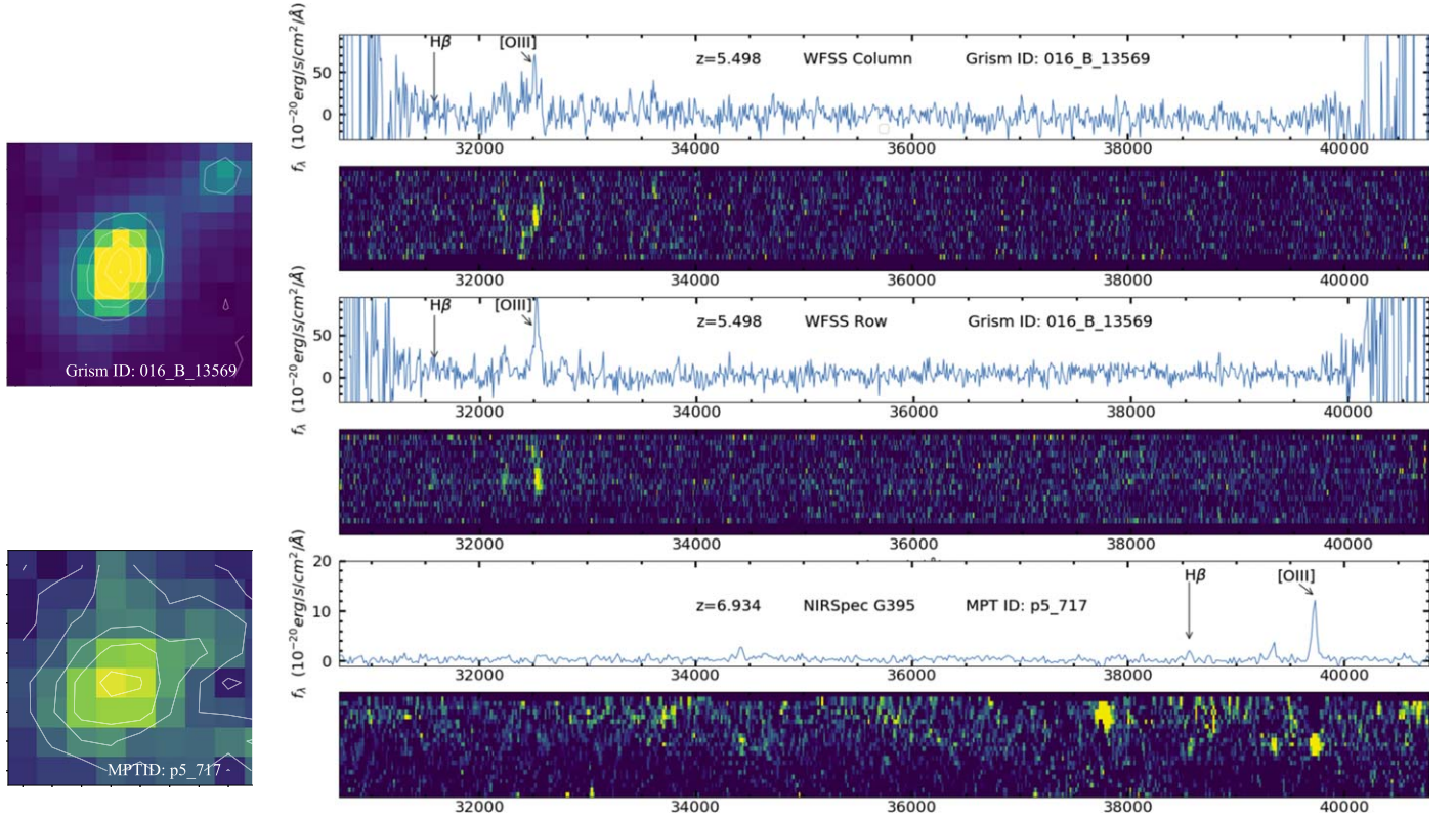
Figure 1. Example of NIRCcam WFSS direct image (left) with 1D/2D column and row WFSS spectra for an example galaxy, 016_B_13569, that is in our [O III]/H \beta sample. Vertical lines in the 1D spectra indicate the emission lines of interest. We also include the direct image and 1D/2D NIRSpect spectra of p5_717 from the G395M filter (bottom).
