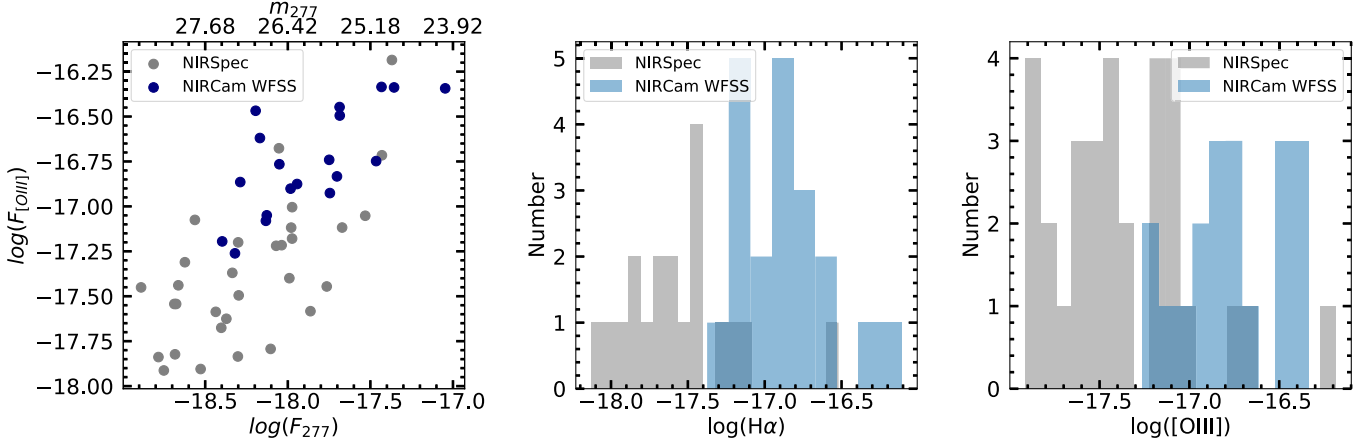
Figure 4. Left: Comparison of the NIRSpec and NIRCcam WFSS measurements of F277W photometric flux and [O\text{ III}] flux. Comparison between emission-line flux from NIRSpec (gray histogram) and NIRCcam WFSS (blue histograms) for H\alpha emission (middle panel) and [O\text{ III}] emission (right panel). Both these emission lines were seen in both instruments. A blind survey like NIRCcam WFSS includes galaxies that have been missed in the targeted NIRSpec observations. The NIRCcam WFSS galaxies tend to have stronger emission lines, due to the higher flux limit.
