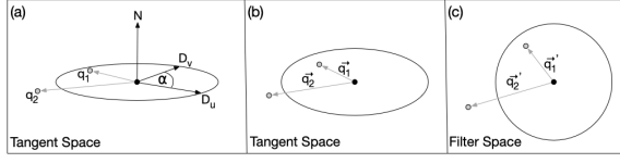
Figure 4: Transformation from tangent space to filter space. (a) In tangent space, the footprint is defined by the normal vector and positional differentials. Vectors connecting the footprint’s center to the query points q_1 and q_2 are constructed. (b) Tangent space is shown along the -N direction for clarity. (c) Vectors \vec{q}_1 and \vec{q}_2 are transformed into filter space using M_p^{-1} . q_1 intersects the footprint since \vec{q}_1' has a magnitude smaller than one.
