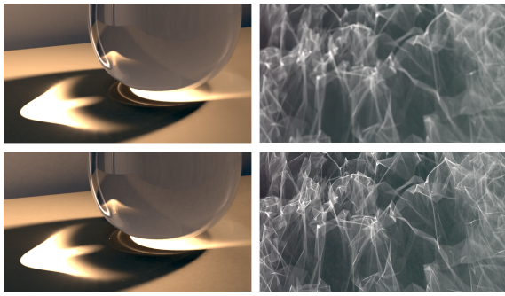
Figure 6: Qualitative comparison of caustics under E-1000K (top-left: RTPM, 100,000 iterations; bottom-left: ARPA, 10,000 iterations; right: RTPM and ARPA, 500 iterations).
