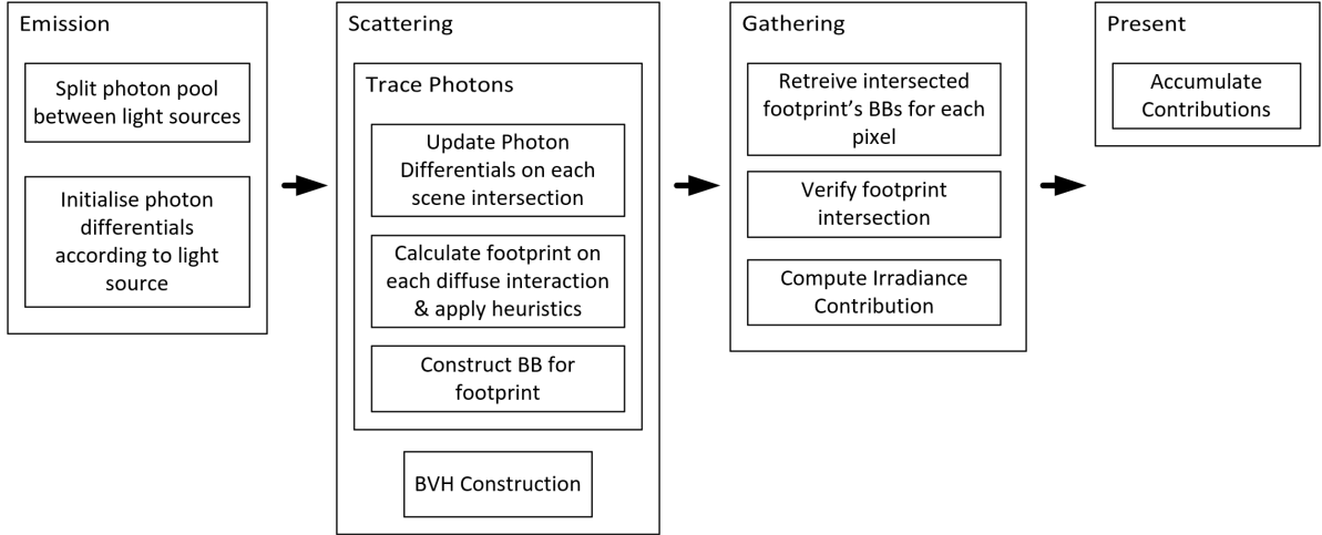
Figure 2: Pipeline illustrating the primary steps for incorporating photon differentials into ray tracing hardware.
