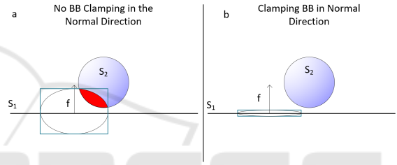
Figure 3: For a photon with an elliptical footprint f , intersecting surface S_1 , (a) uses an un-clamped bounding box in the normal direction which results in light leaks to surface S_2 (shaded in red), while (b) clamps the bounding box in the normal direction to reduce the chances of light leaks.
