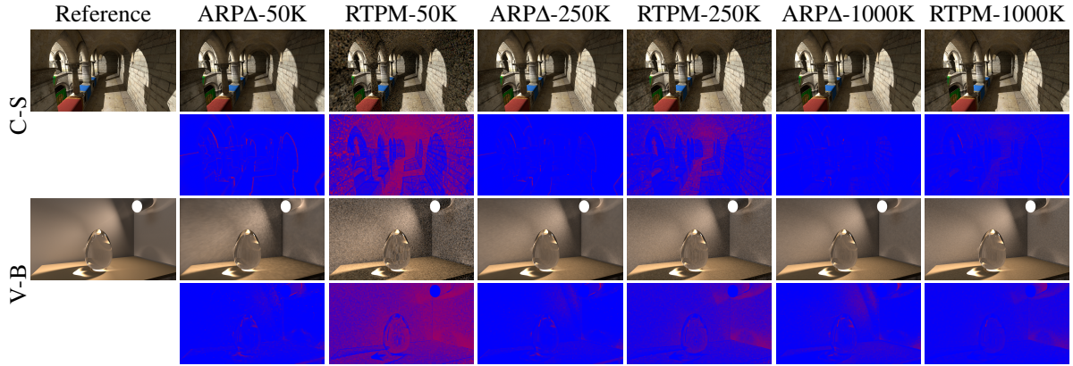
Figure 5: Renders and the corresponding SSIM heatmaps at the ten-second mark for C-S and V-B, for all three experiment configurations (E-50K, E-250K and E-1000K).
