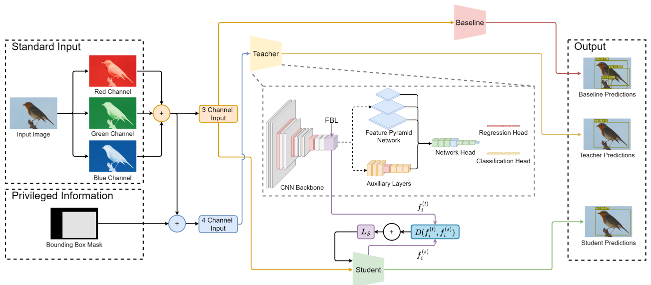
Figure 3.3 Detailed architecture of the training setup showing the teacher network receiving both RGB images and privileged input channels. The student network processes only RGB data but is trained with additional supervision through knowledge distillation. A baseline RGB-only model is included for comparison.
