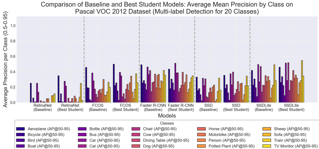
Figure 4.14 Comparison between the baseline and best-performing student models based on mean average precision by class on the Pascal VOC 2012 dataset for multi-label detection of 20 object classes.
