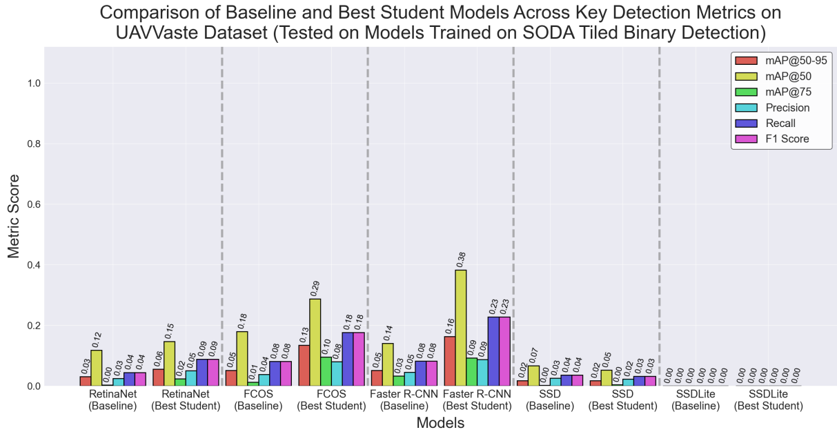
Figure 4.12 Comparison of baseline and best-performing student models on key detection metrics using the UAVWaste dataset. The evaluated models were trained on the 3 \times 3 tiled SODA dataset across all altitudes for binary litter detection.
