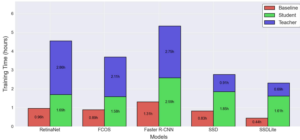
Figure 4.16 Comparison of model training times on the Pascal VOC 2012 dataset for multi-label detection of 20 object classes.
