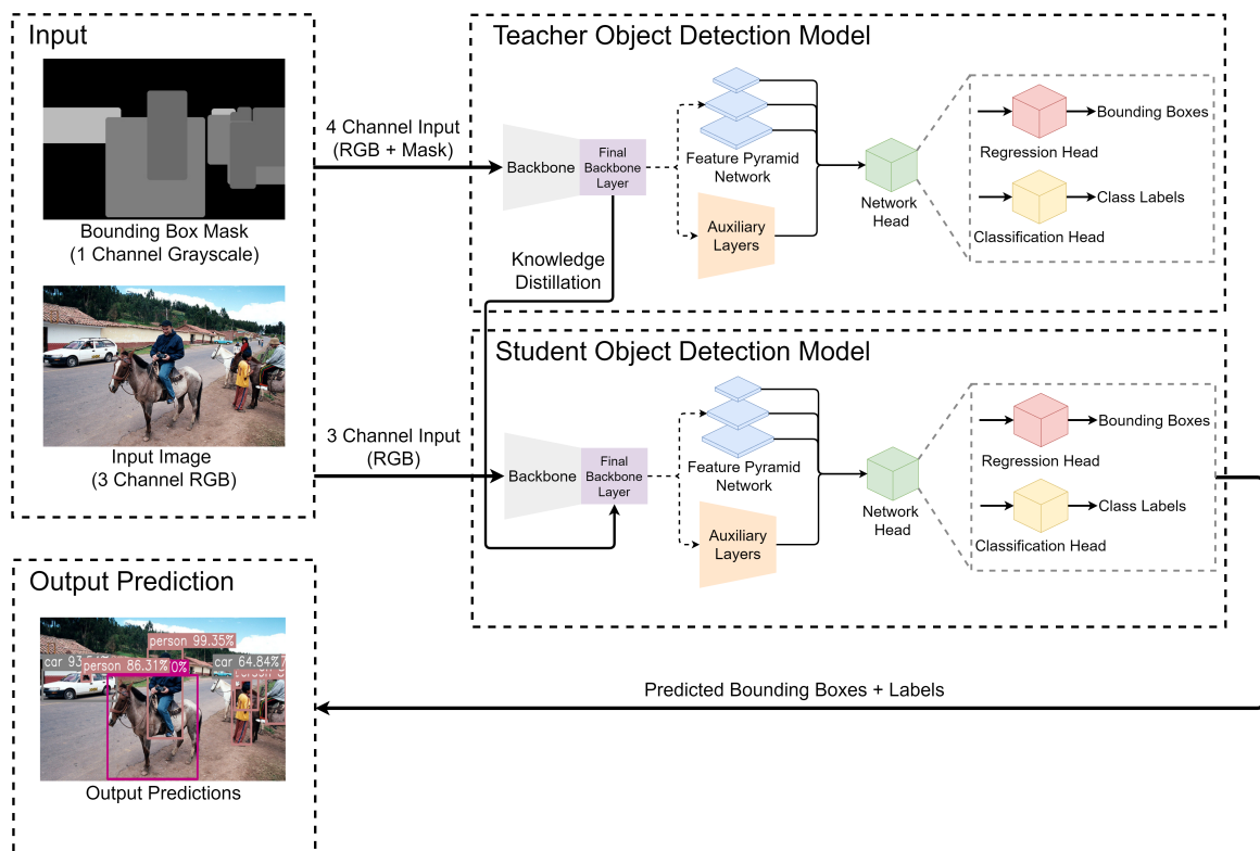
Figure 3.2 General architecture for integrating the LUPI paradigm into any object detection model. The diagram illustrates the incorporation of both RGB images and bounding box masks as inputs to the teacher network, the use of a standard RGB input for the student network, the selection of the final backbone layer for knowledge distillation, and the generation of output predictions from the student model.
