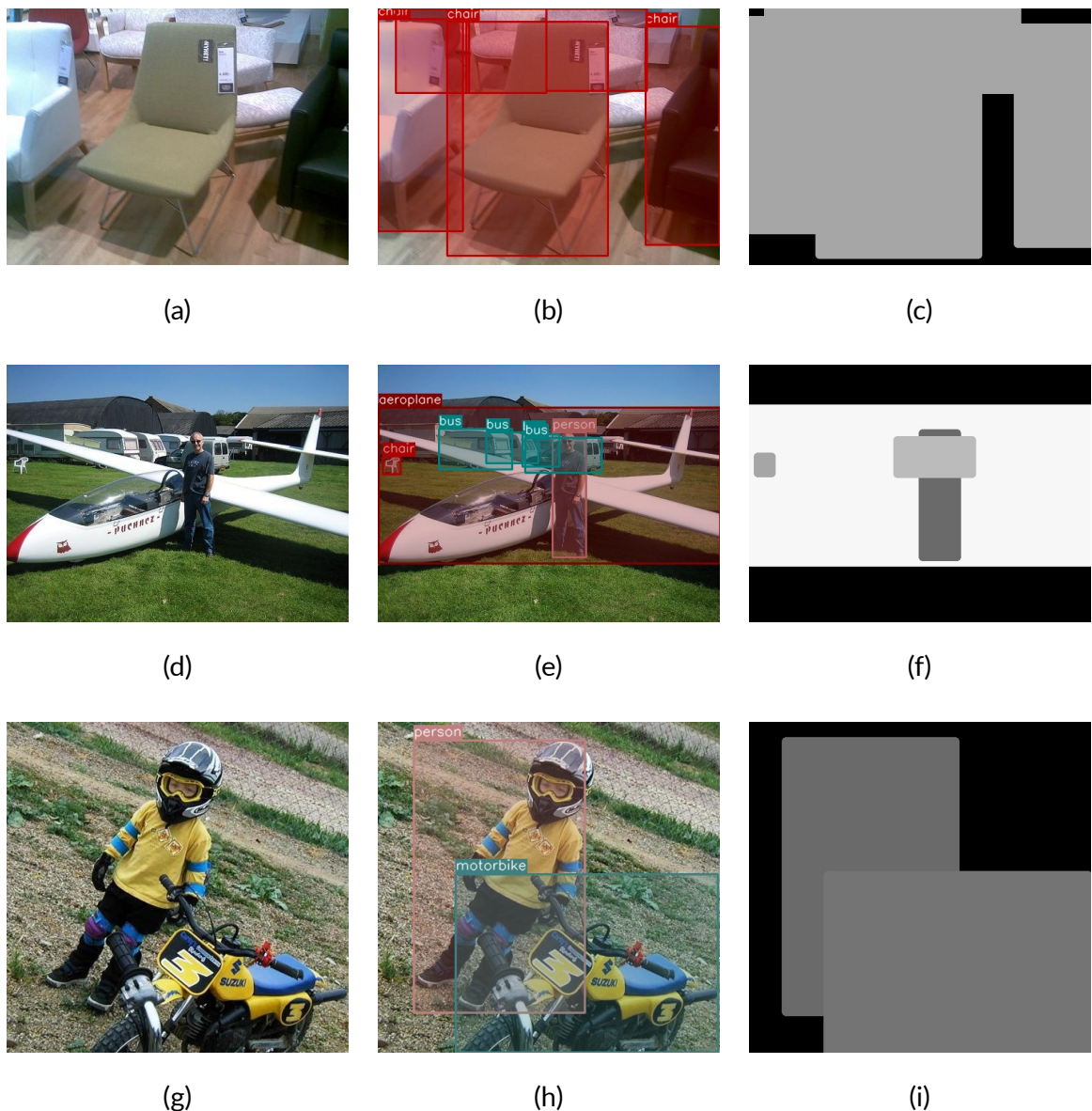
Figure 4.24 Examples of failure cases in privileged information generation. Subfigures (a), (d), and (g) show original images from the Pascal VOC 2012 dataset, while (b), (e), and (h) display the corresponding images with overlaid ground truth annotations. Subfigures (c), (f), and (i) present the privileged information for these cases.
