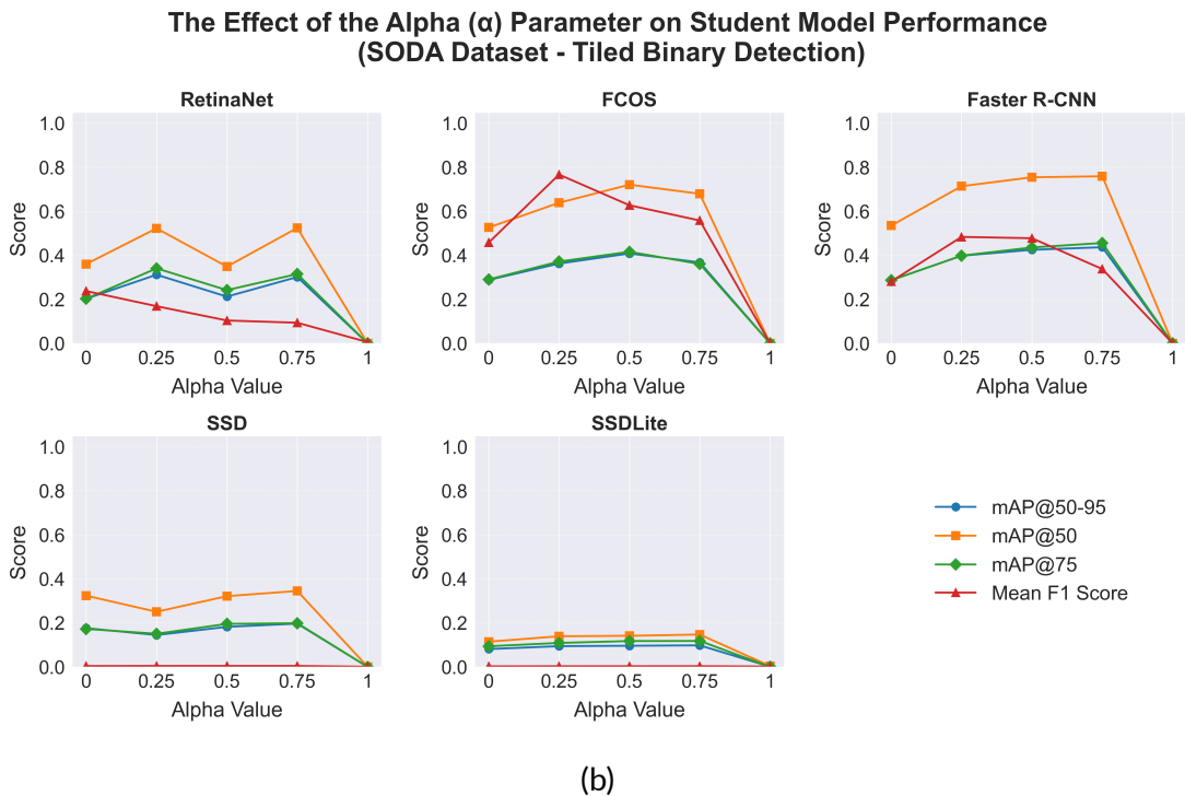
Figure 4.17 Assessing the impact of the alpha ( \alpha ) parameter on student model performance. (a) shows results for the SODA dataset at a 1-metre altitude for binary litter detection, while (b) presents results on the 3 \times 3 tiled SODA dataset across all altitudes for binary litter detection.
