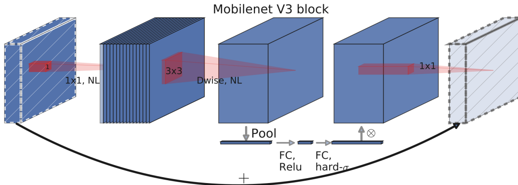
Figure 2.7 MobileNetV3 architecture. (Source: [74])
