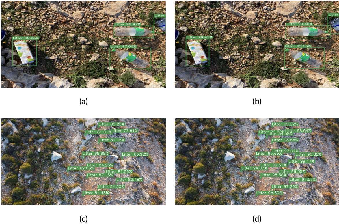
Figure 4.19 Sample predictions on test subset images from detection models trained on the SODA dataset. Subfigures (a) and (c) show outputs from the baseline models, while (b) and (d) present predictions from their corresponding student models. Subfigures (a) and (b) illustrate RetinaNet results at an altitude of 1 metre; (c) and (d) show outputs from Faster R-CNN.
