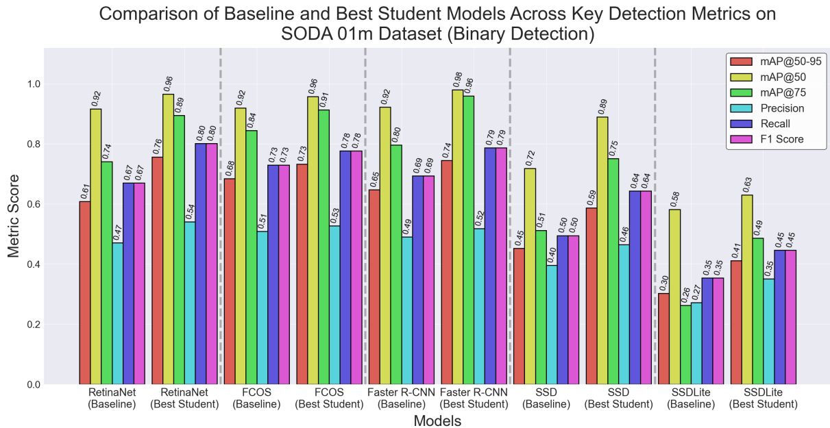
Figure 4.3 Comparison between the baseline and the best-performing student models across key detection metrics on the SODA dataset at a 1-metre altitude for binary litter detection.
