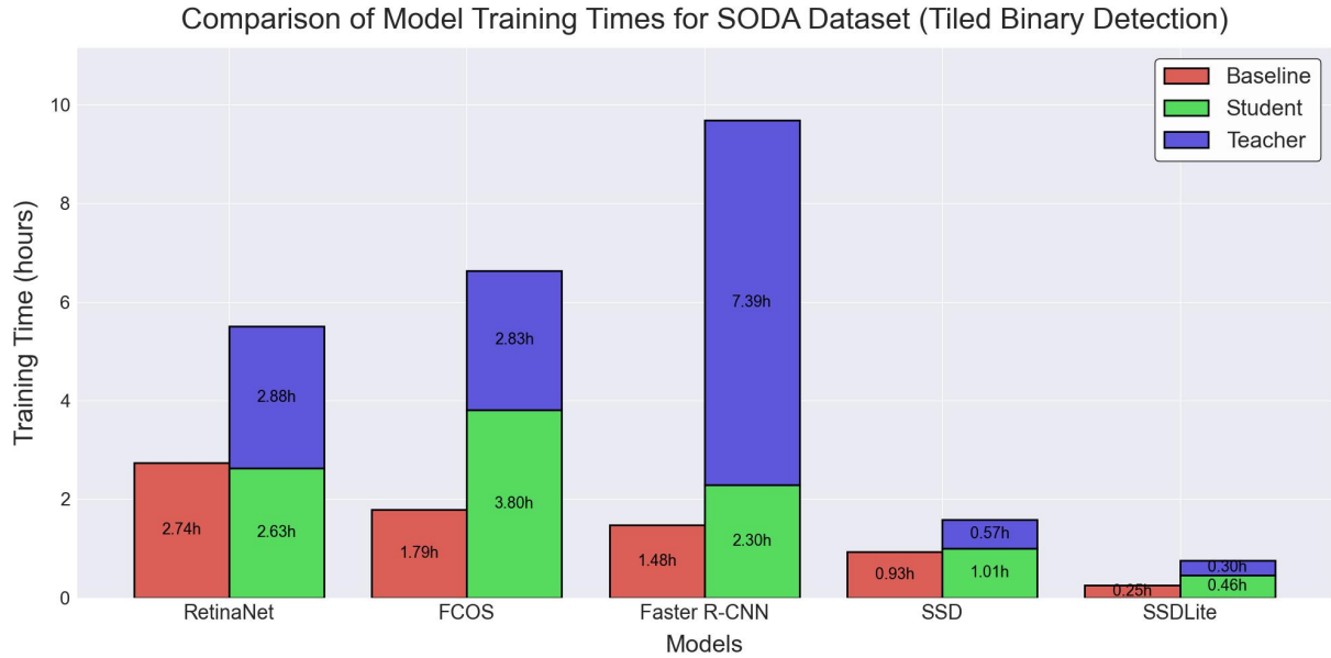
Figure 4.6 Comparison of model training times on the 3 \times 3 tiled SODA dataset across all altitudes for binary litter detection.
