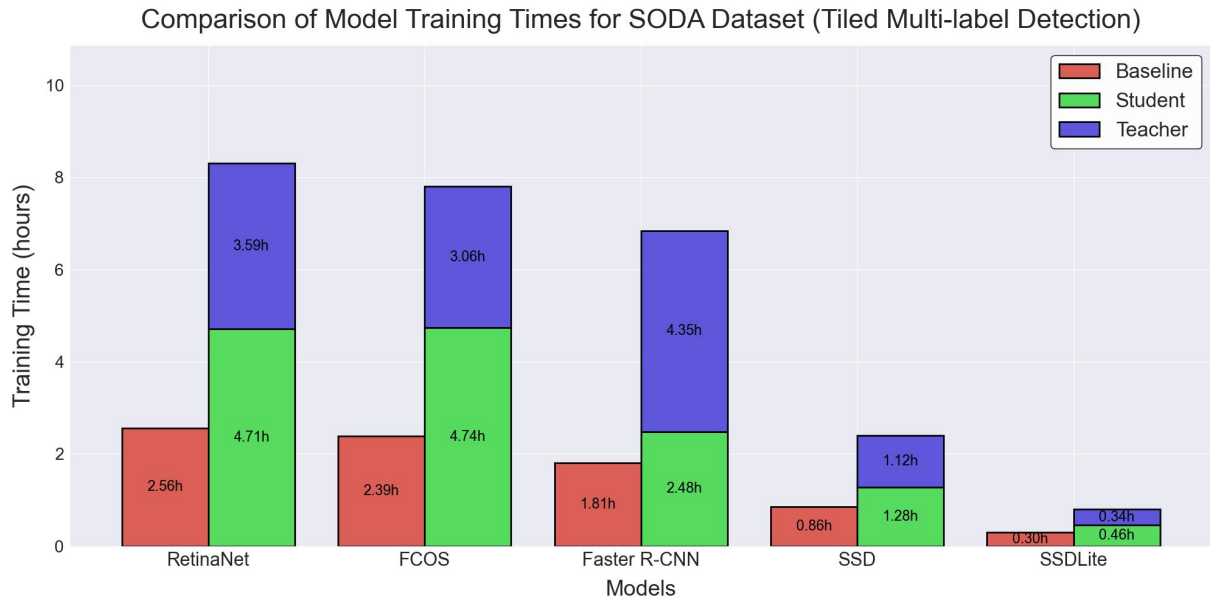
Figure 4.10 Comparison of model training times on 3 \times 3 tiled SODA dataset across all altitudes for multi-label litter detection.
