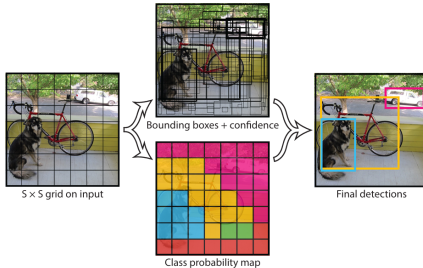
Figure 2.3 YOLOv1 pipeline. (Source: [61])
