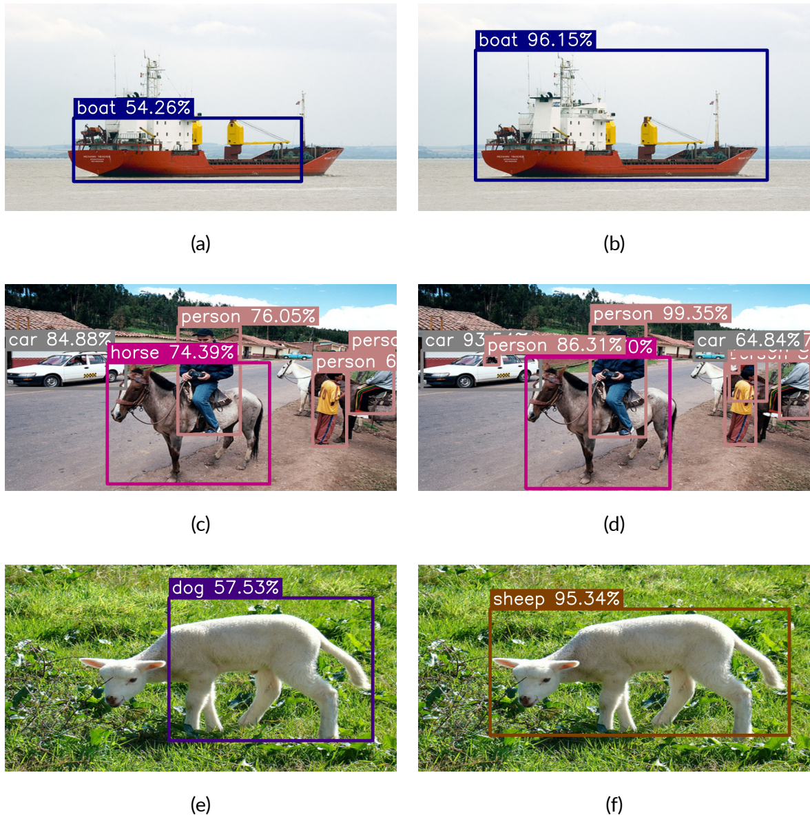
Figure 4.22 Sample predictions from the best-performing detection model, Faster R-CNN, trained on the Pascal VOC 2012 dataset. Subfigures (a), (c), and (e) show outputs from the baseline model, while (b), (d), and (f) present predictions from the corresponding student model.
