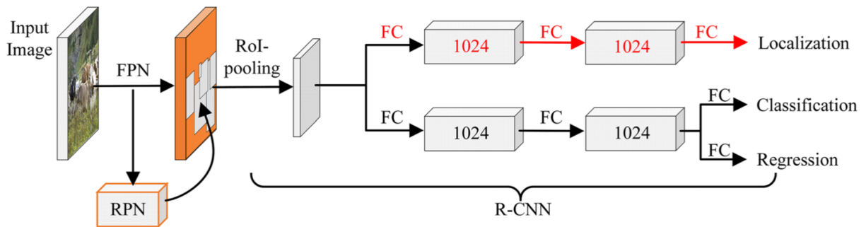
Figure 2.10 Faster R-CNN architecture with ResNet-50 backbone and integrated FPN, demonstrating a unified two-stage detection pipeline for proposal generation, classification, and bounding box regression. (Source: [81])
