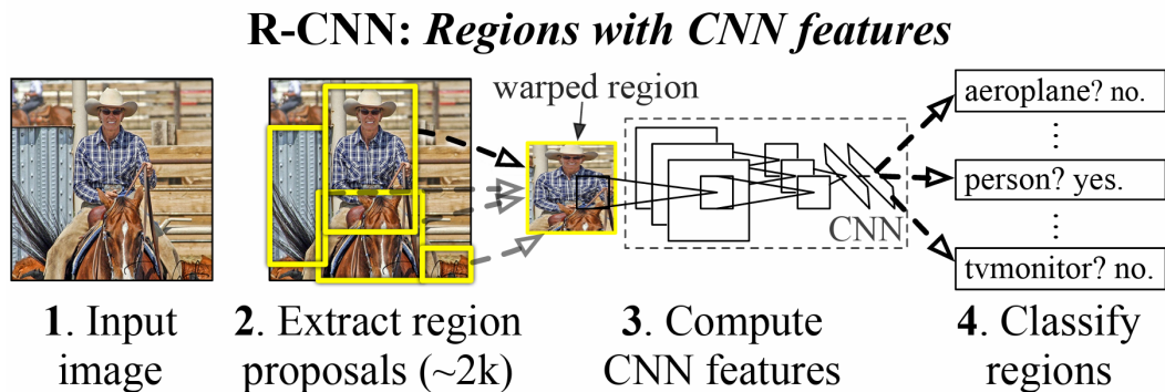
Figure 2.9 R-CNN architecture. (Source: [76])
