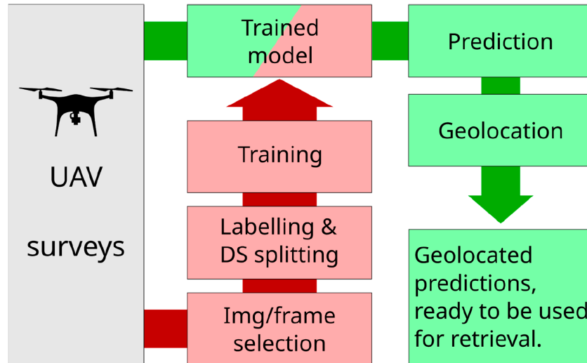
Figure 2.30 The system architecture of the real-time UAV beach litter monitoring and geolocation system, highlighting the two main pipelines: training (in red) and prediction (in green). (Source: [126])
