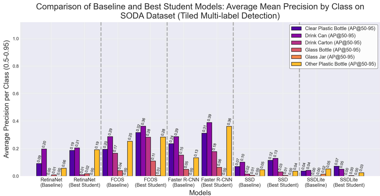
Figure 4.8 Comparison between the baseline and best-performing student models based on mean average precision by class on the 3 \times 3 tiled SODA dataset across all altitudes for multi-label litter detection.
