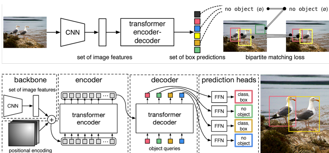
Figure 2.12 DETR architecture. (Source: [9])
