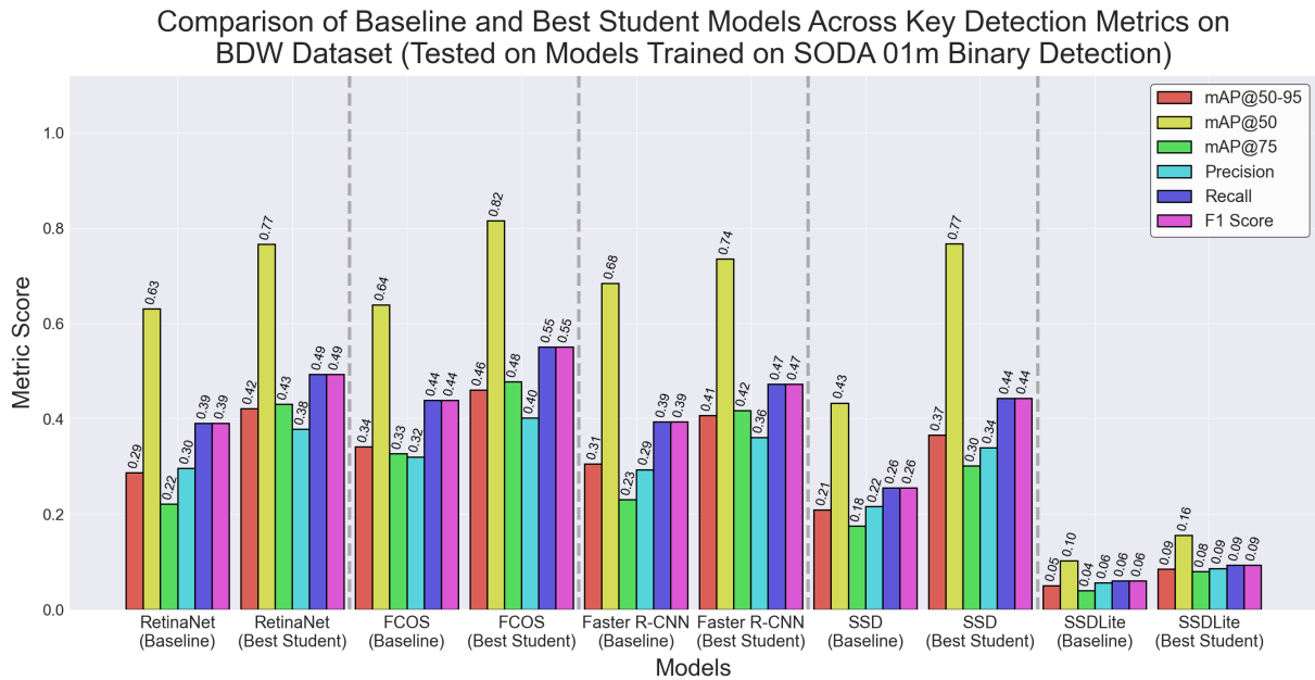
Figure 4.11 Comparison of baseline and best-performing student models on key detection metrics using the BDW dataset. The evaluated models were trained on the SODA dataset captured at 1-metre altitude for binary litter detection.
