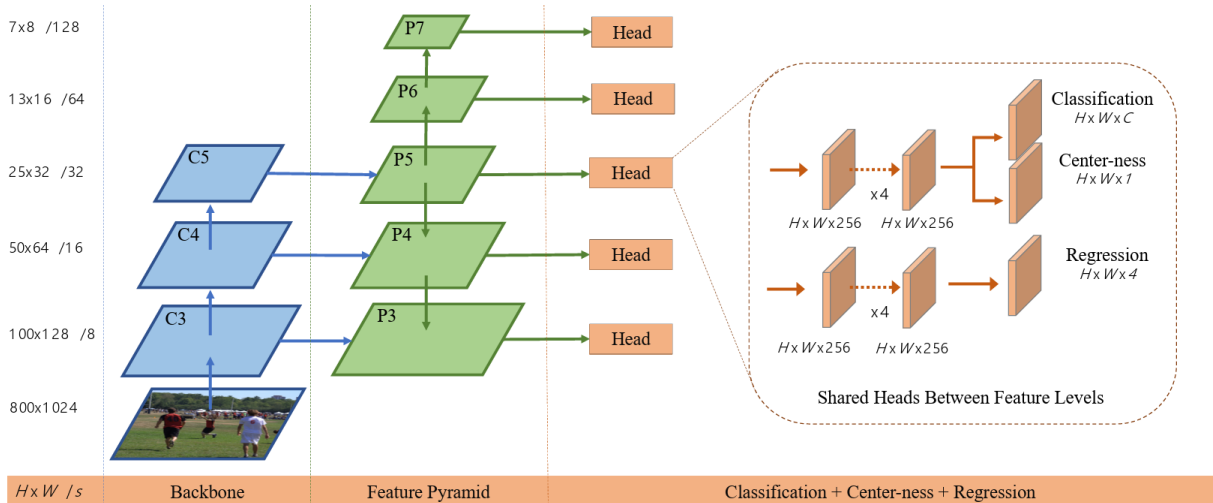
Figure 2.8 FCOS architecture. (Source: [75])
