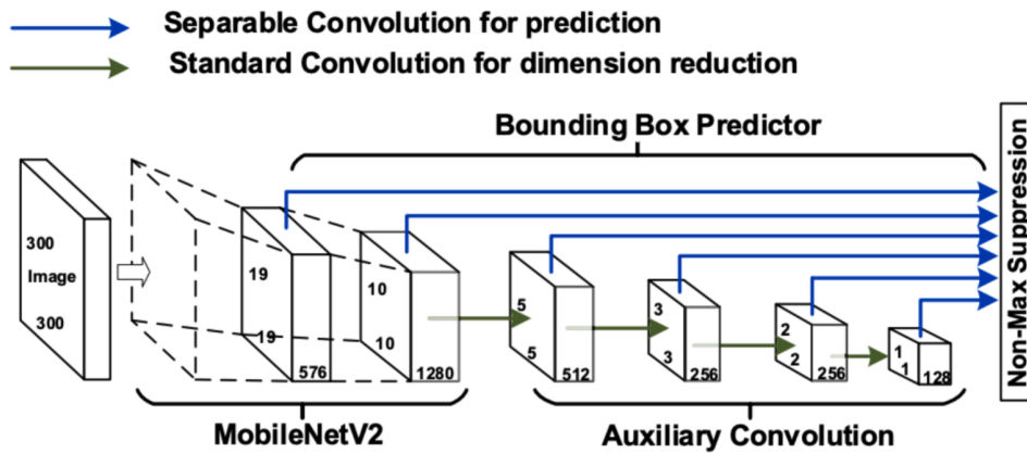
Figure 2.6 MobileNetV2-SSDLite architecture. (Source: [73])
