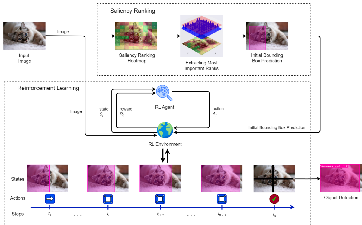
Figure 2.14 Architecture of a reinforcement learning-based object detection framework for iterative object localisation. (Source: [58])
