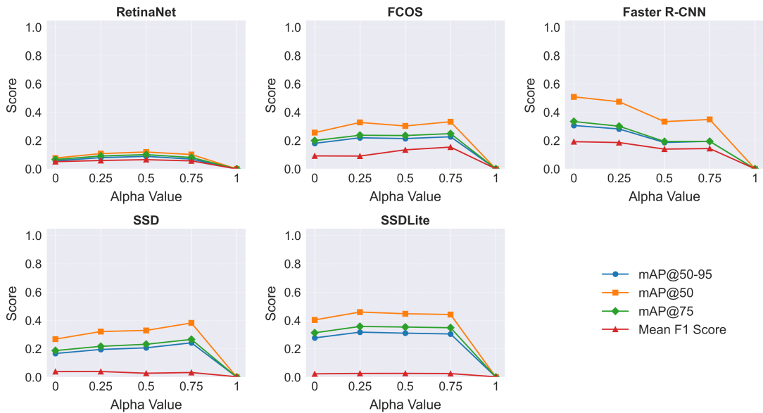
The Effect of the Alpha ( \alpha ) Parameter on Student Model Performance (Pascal VOC 2012 Dataset - Multi-label Detection)
