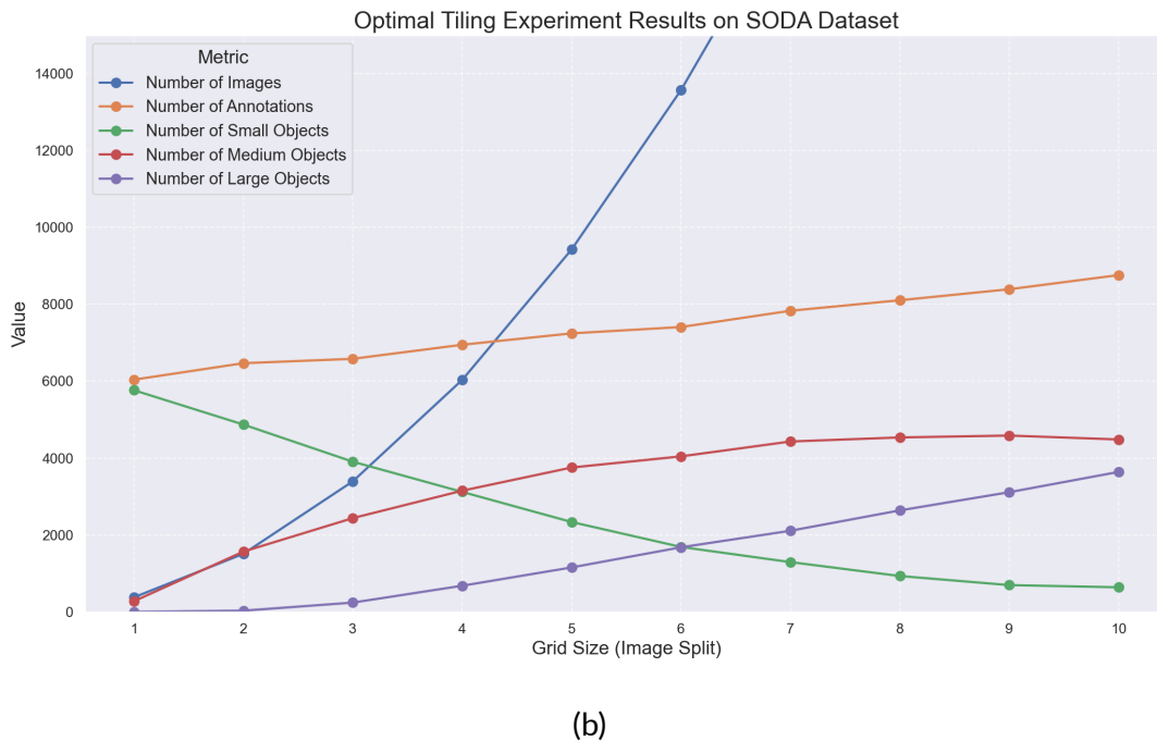
Figure 4.1 Optimal tiling experiment results on the SODA dataset, illustrating the increase in the number of images and annotated objects as the grid size increases. (a) Results over the full altitude range (1–30 metres), and (b) results on a subset of altitudes (5–30 metres) from the SODA dataset.
