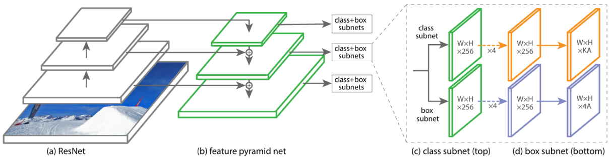
Figure 2.5 RetinaNet architecture. (Source: [71])
