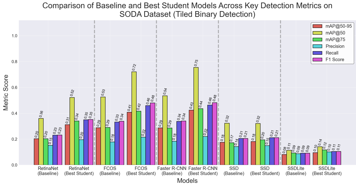
Figure 4.5 Comparison between the baseline and best-performing student models across key detection metrics on the 3 \times 3 tiled SODA dataset across all altitudes for binary litter detection.
