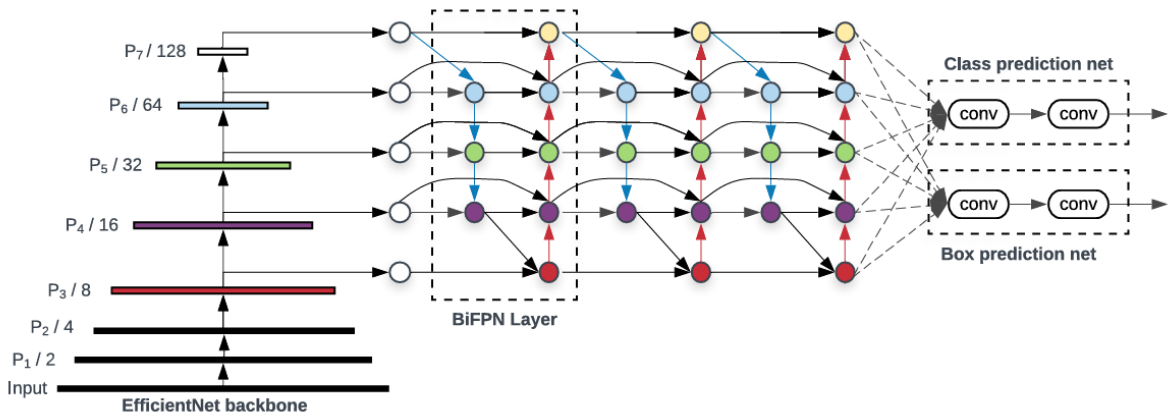
Figure 2.11 EfficientDet architecture. (Source: [84])
