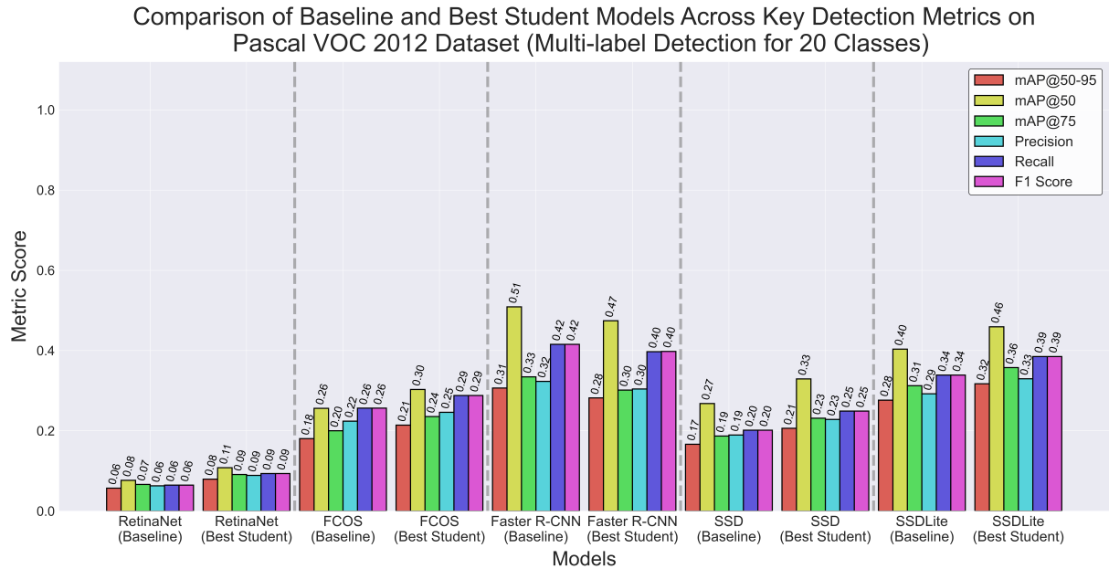
Figure 4.13 Comparison between the baseline and best-performing student models across key detection metrics on the Pascal VOC 2012 dataset for multi-label detection of 20 object classes.
