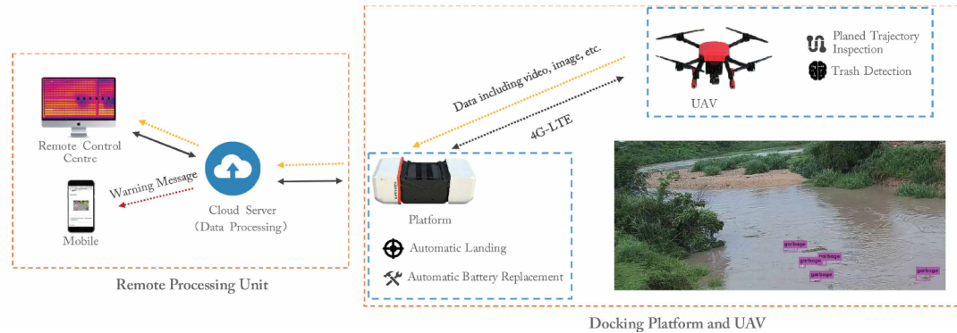
Figure 2.18 Block diagram of the automated SuperDock system. (Source: [114])
