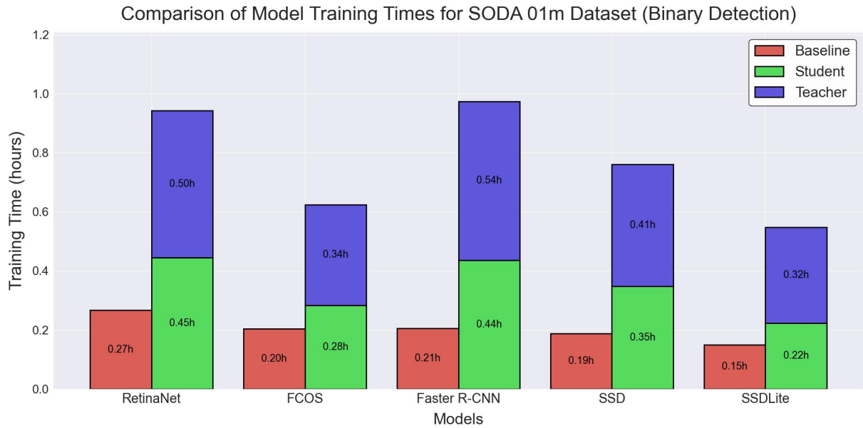
Figure 4.4 Comparison of model training times on the SODA dataset at a 1-metre altitude for binary litter detection.
