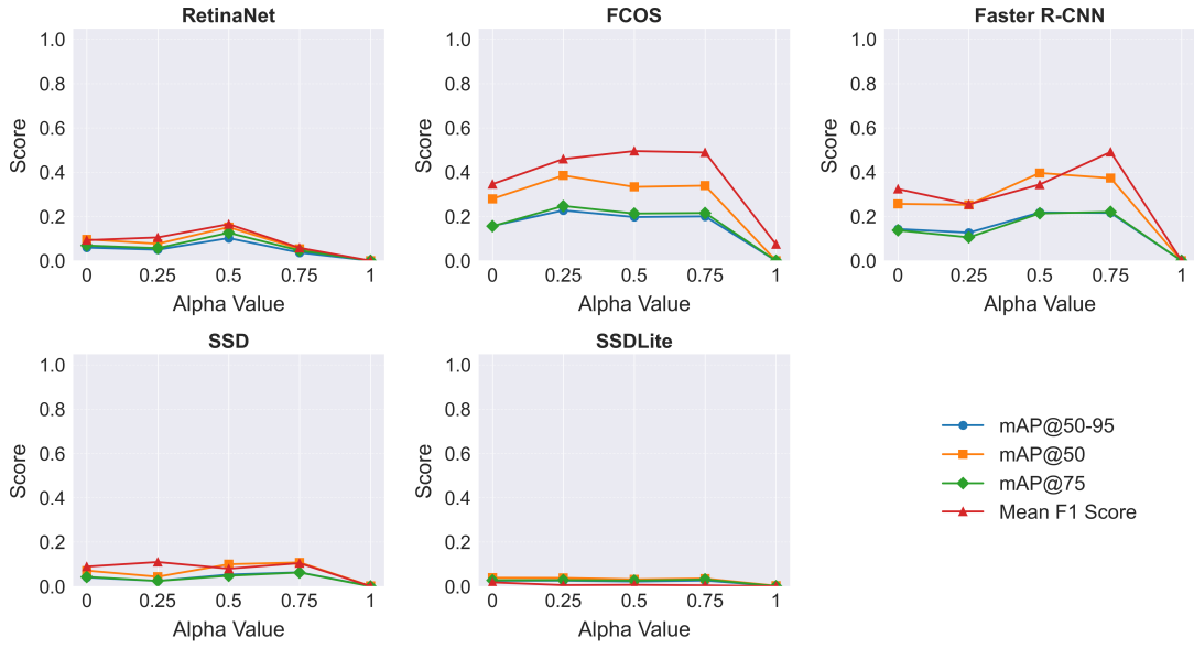
The Effect of the Alpha ( \alpha ) Parameter on Student Model Performance (SODA Dataset - Tiled Multi-label Detection)
