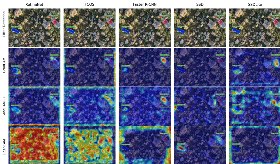
Visual Comparison of Object Detection Models Using Various CAM Methods on the SODA 01m Altitude Dataset (Student Models)
