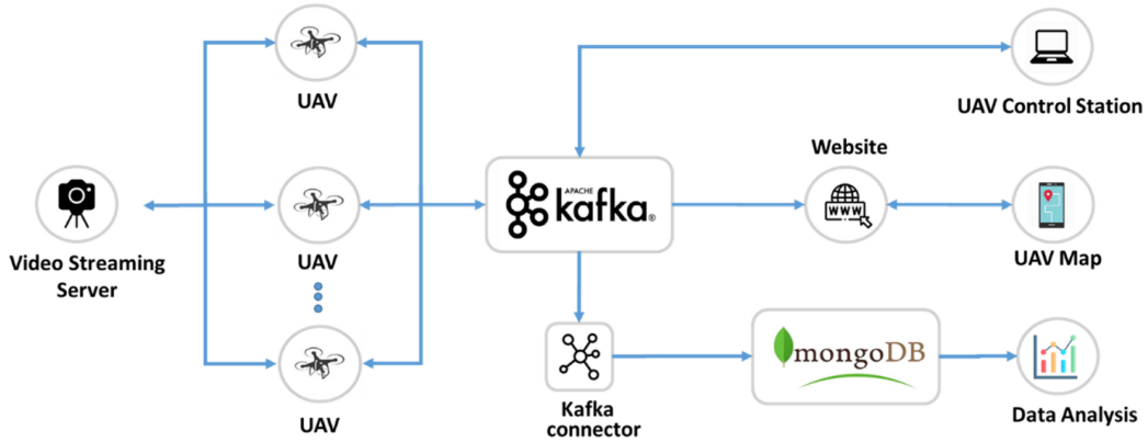
Figure 2.27 The system architecture of the real-time UAV trash monitoring system. (Source: [124])
