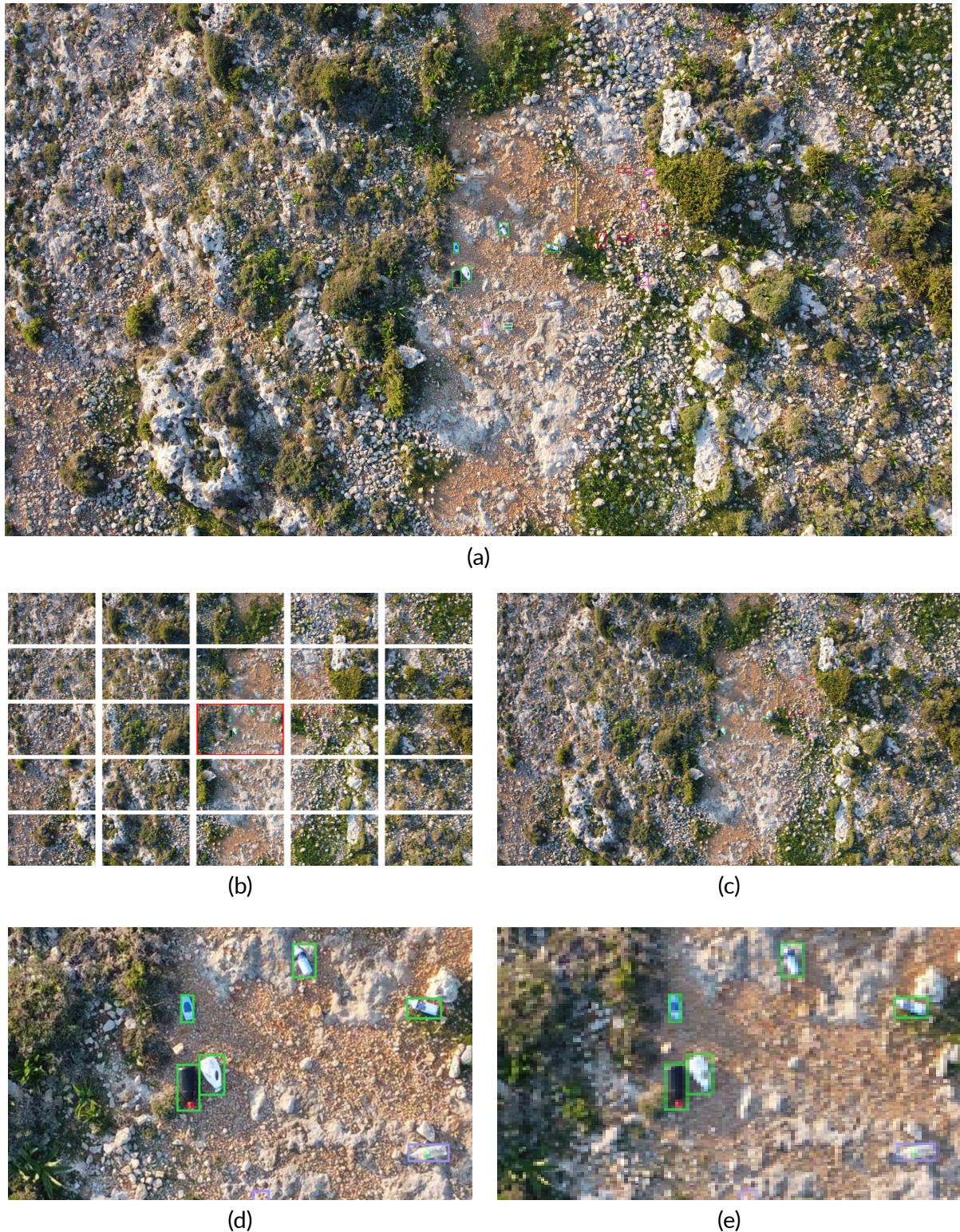
Figure 3.4 Visual illustration highlighting the need for tiling. (a) Annotated image of litter captured at 15 metres altitude from the SODA dataset [13]; (b) 5 \times 5 tiling of the original image, with each tile resized to 640 \times 640 pixels; (c) original image resized directly to 640 \times 640 pixels; (d) the 13 th tile from the tiling approach, resized; (e) the corresponding region extracted from the non-tiled image.
