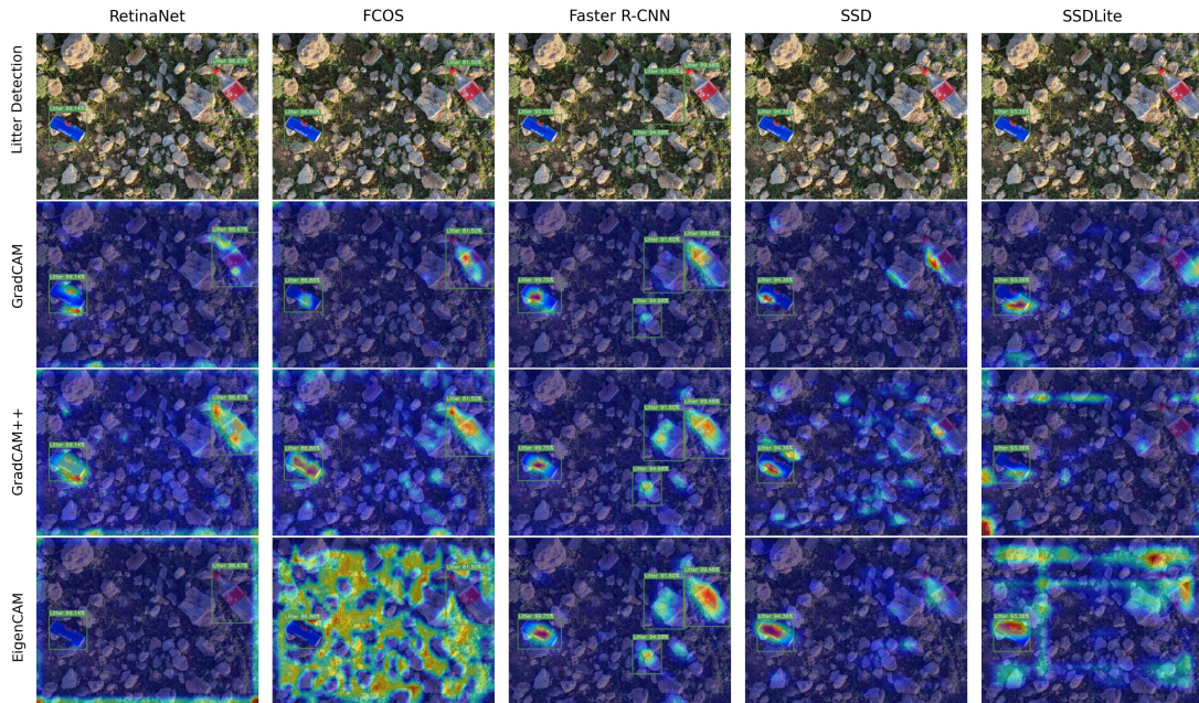
Visual Comparison of Object Detection Models Using Various CAM Methods on the SODA 01m Altitude Dataset (Baseline Models)
