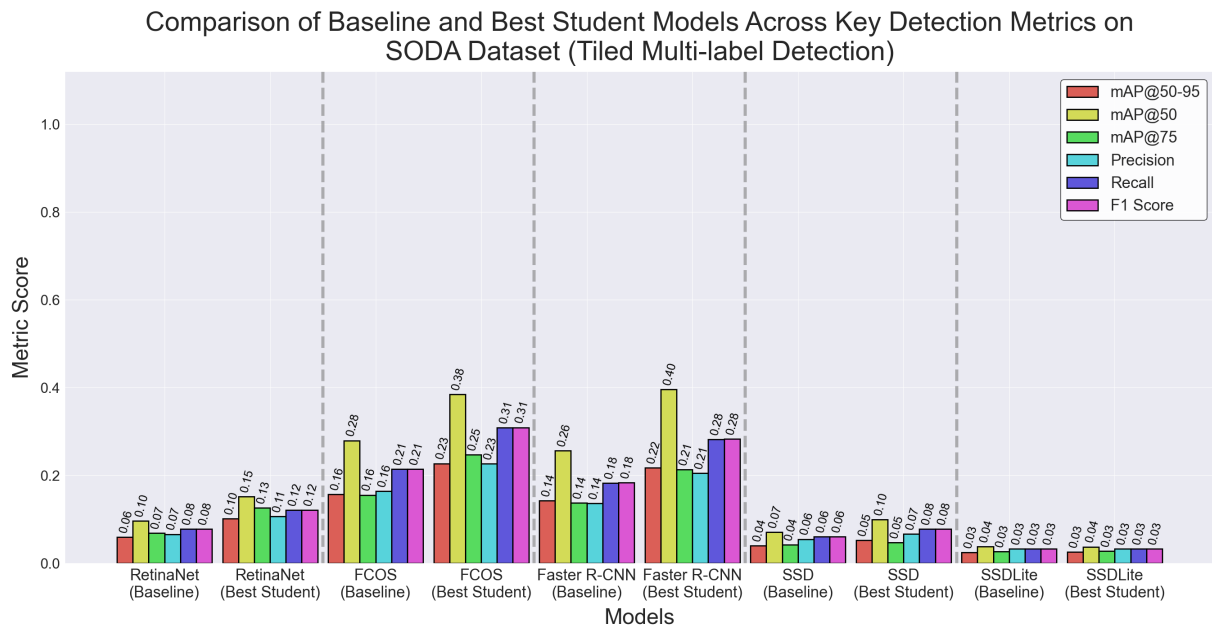
Figure 4.7 Comparison between the baseline and best-performing student models across key detection metrics on the 3 \times 3 tiled SODA dataset across all altitudes for multi-label litter detection.
