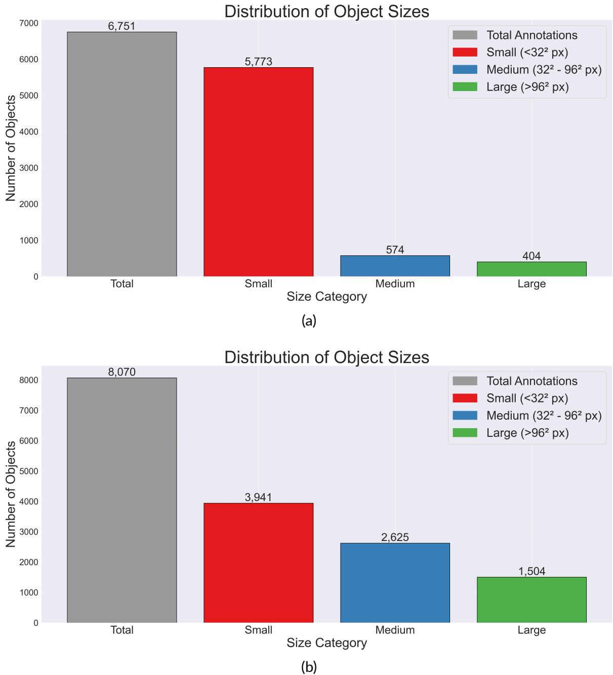
Figure 3.8 SODA dataset object size distribution: (a) before 3 \times 3 tiling, and (b) after 3 \times 3 tiling.
