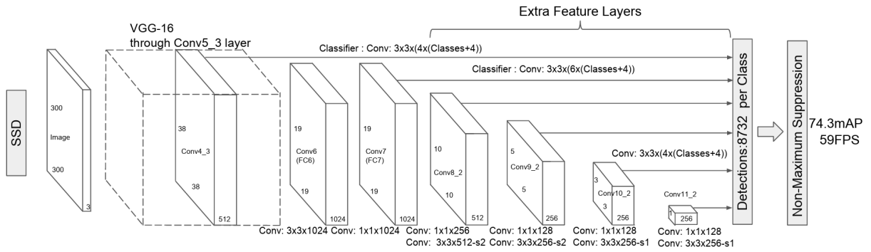
Figure 2.4 SSD architecture. (Source: [70])
