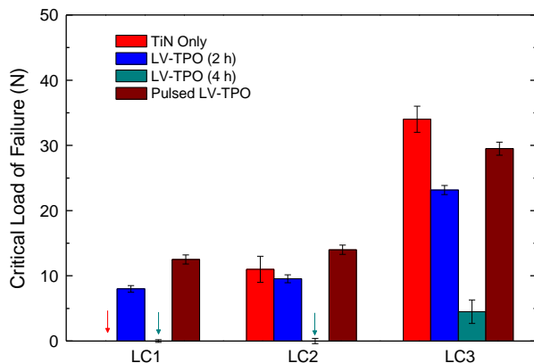
Fig. 4. Critical loads for failure of a 2.8 µm TiN coating deposited on untreated and different pre-oxidised Ti-6Al-4V samples. All TPO processes were held at 700 °C.
