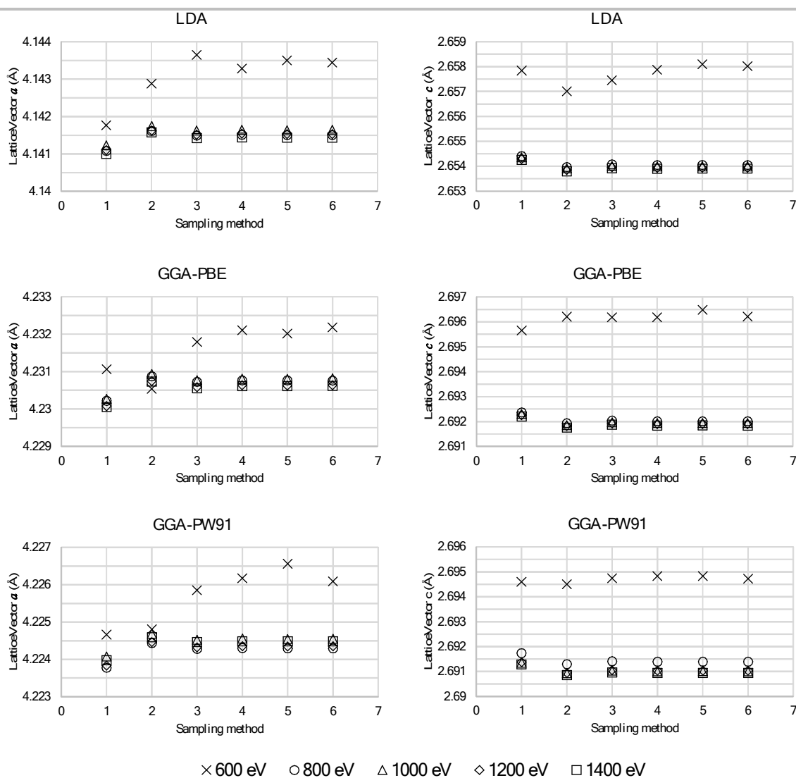
Figure S1: Convergence testing of the three functional studied (LDA, GGA-PBE and GGA-PW91). Convergence testing was carried out with respect to sampling mesh as well as the cut off energy. Sampling methods represent the Monkhorst-Pack k -point grid as follows; 1: 3x3x5, 2: 4x4x6, 3: 5x5x7, 4: 6x6x8, 5: 7x7x9, 6: 8x8x10.
