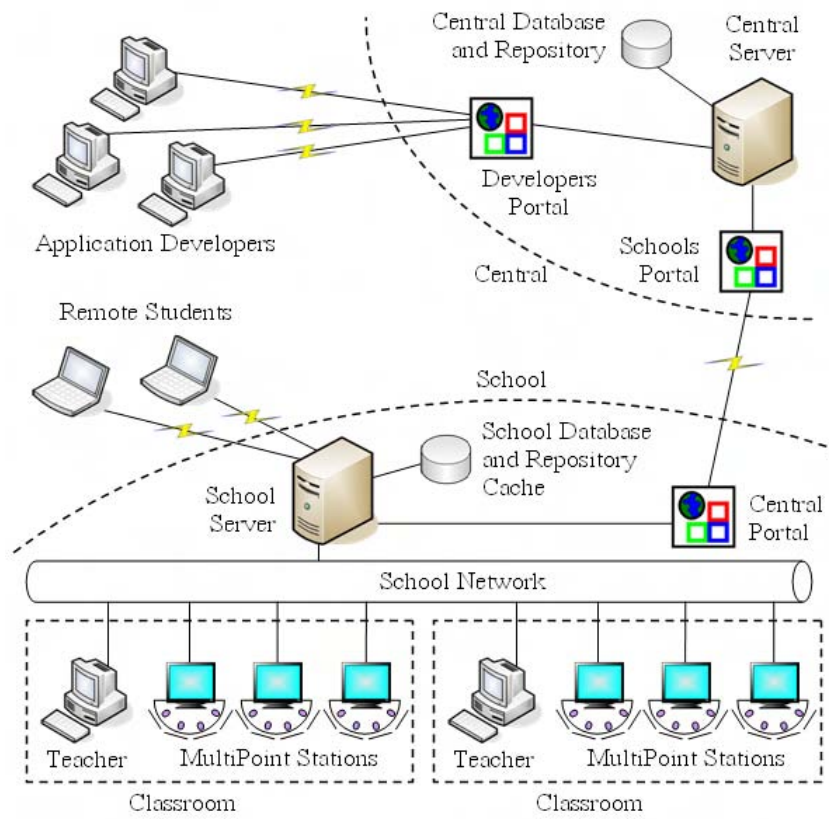
Fig. 2: System Architecture
