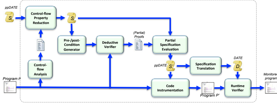
Fig. 4. High-level description of the StaRVOOrS framework workflow enriched with control-flow analysis
