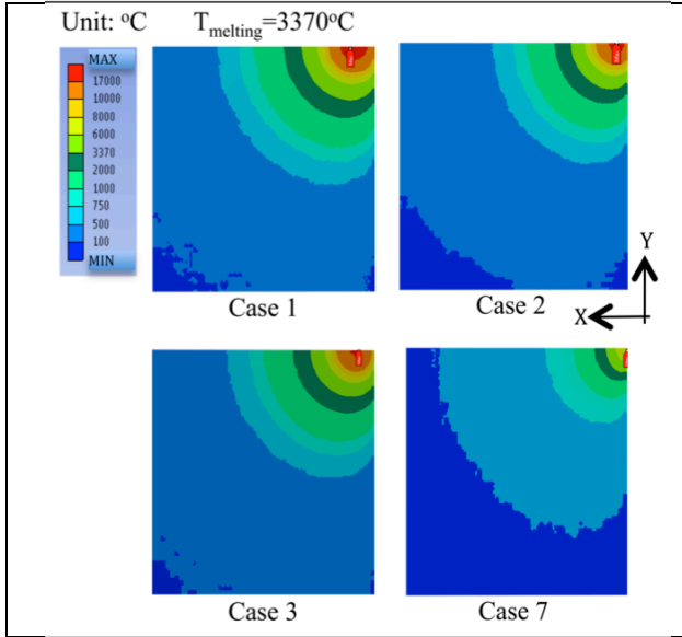
Figure 4: Comparison of the cross-sectional temperature distribution at T_{\max} -slice just after the impact at 7TeV. Note that the region from the dark green edge towards the corner is above the melting temperature.
