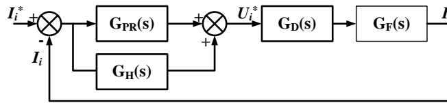
Fig. 3 The PR Current Control with Harmonic Compensators
