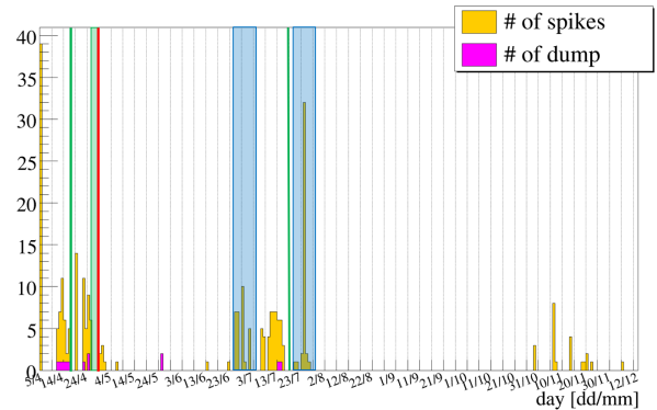
Figure 9: The number of spikes observed at the ULO location and induced beam dump as a function of the day, during the whole 2015 run. Days in which a thermal cycle of the beam screen was performed are shown by green lines, while the day in which the fixed bump was deployed is indicated by a red line, and the scrubbing runs are in blue.
