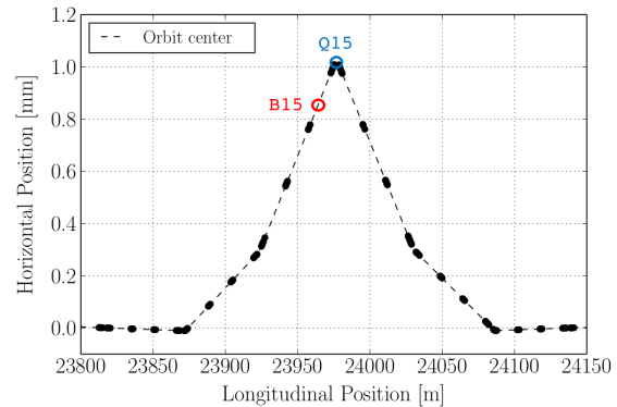
Figure 1: Local orbit bump (3 correctors) for shifts in the horizontal plane. Q15 is enlightened in blue, while B15 in red.
