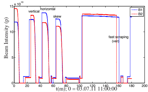
Figure 1: Intensity during the beam distribution MD, July 2011. It can be seen that B1 and B2 were scraped away in parallel with a delay of 2 seconds between the movement of the respective primary collimators. The fast and slow full beam scrapings are labelled in the plot accordingly.
