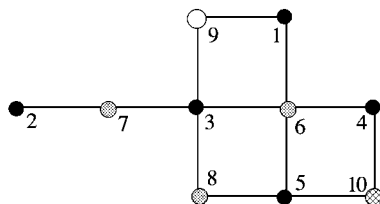
FIG. 5.2. Two SCs with core \overline{K_5} and overlapping peripheries.
