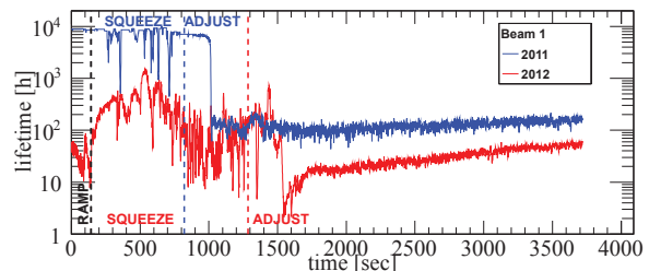
Figure 6: Lifetime as function of time for a typical fill in 2012 and 2011 (fill numbers 2712 and 1732).
