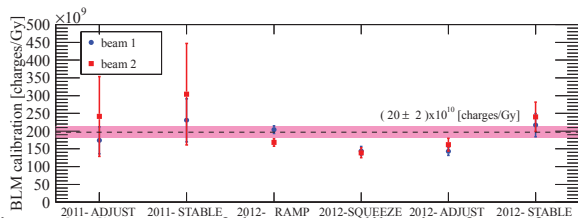
Figure 3: Summary of the BLM calibration factor for different beam modes in 2011 and 2012.
