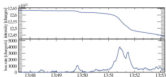
Figure 1: Intensity (top) and loss rate (bottom) during the adjust of fill 2479 for Beam 1 as a function of time.
