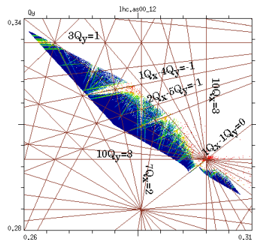
Figure 1: FMA analysis for the case without any errors. For 7 th turn pulsing the 7Q_x resonance is driven and for 10 th turn pulsing the 10Q_{x/y} .
