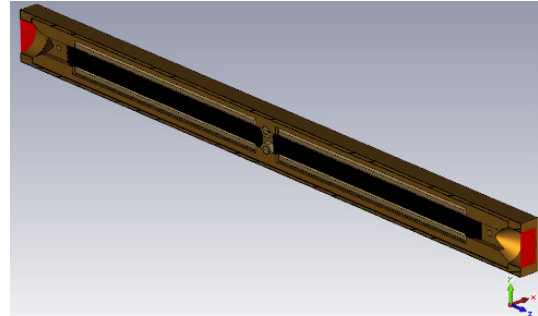
Figure 1: Jaw model of the mock-up collimator with in-jaw BPM buttons [7].
