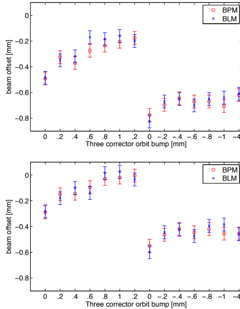
Figure 5: Beam offset measured with the in-jaw BPMs (red circles) and the BLM method (blue crosses) for the downstream (top) and upstream (bottom) ends of the collimator versus the expected amplitude of a three corrector orbit bump.
