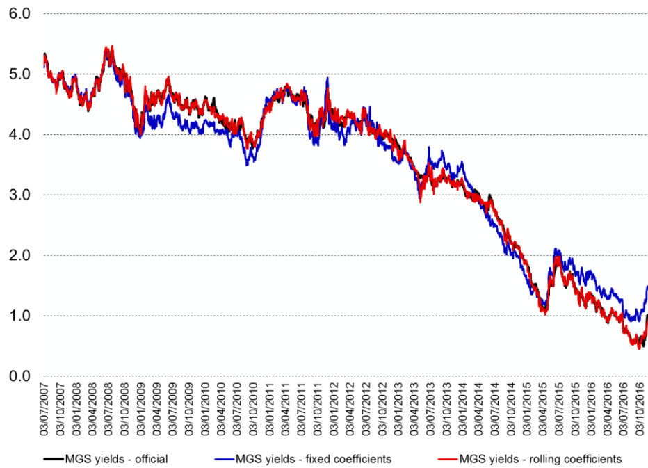
Figure 4: MGS yields, actual and benchmarked on euro area yields
