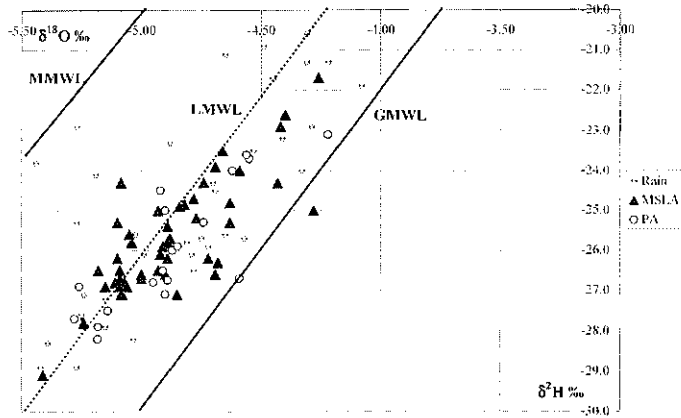
Fig. 2 ^{18}\text{O} vs ^2\text{H} in rain and groundwater, from Malta. Summer evaporated rainwater and groundwater mixed with seawater are not displayed. MSLA: Mean Sea Level Aquifer. PA: Perched Aquifer. The three lines with a slope of 8 display the global (GMWL), local (LMWL) and Mediterranean (MMWL) relationships.
