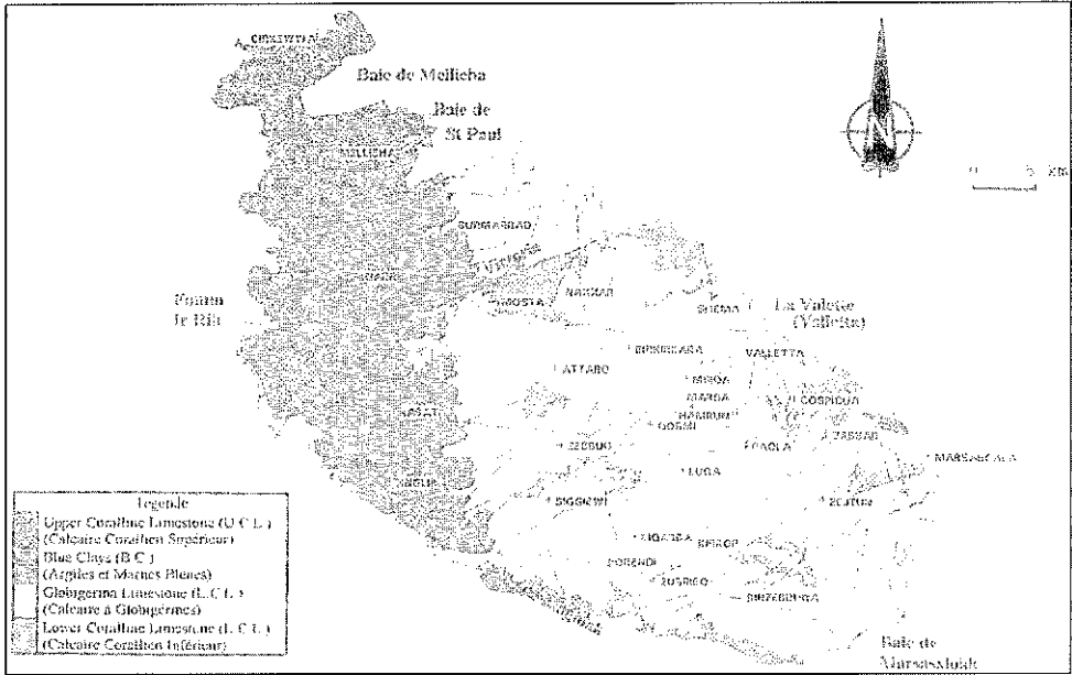
Fig. 1 Geological map of Malta Island.
