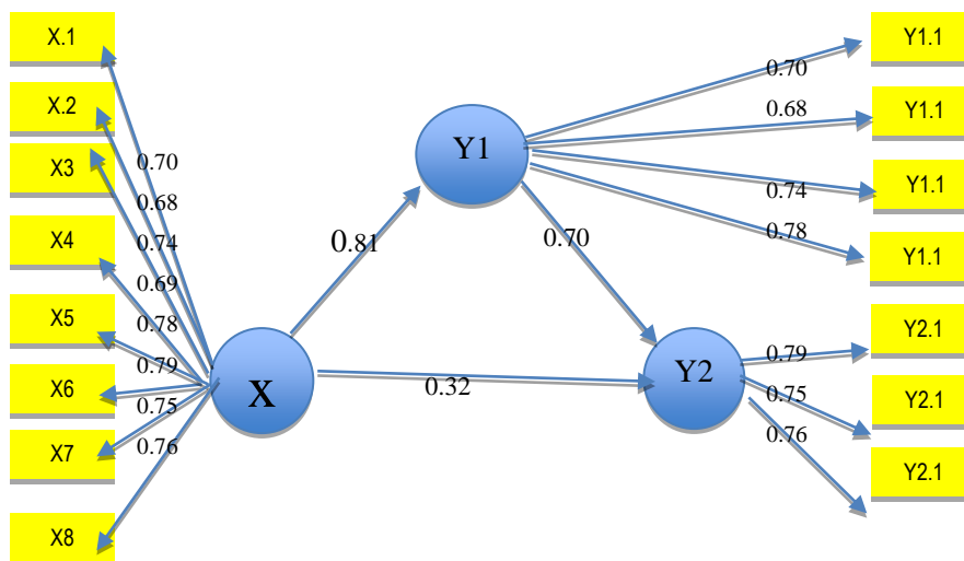
Figure 2. T-Test Diagram
