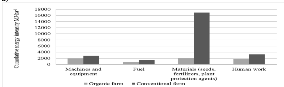
Figure 7. Values of cumulative energy intensity (a) and emergy (b) applied in the conventional and organic cultivation of winter wheat
