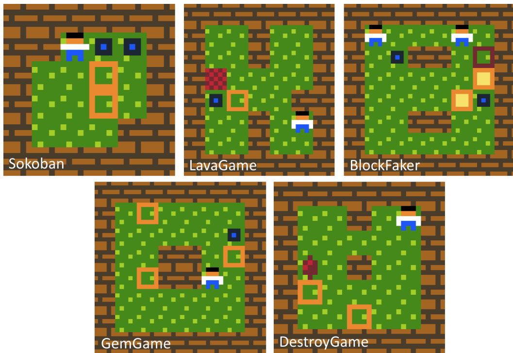
Figure 5.10: Examples of the generated levels using GA with random initialization
