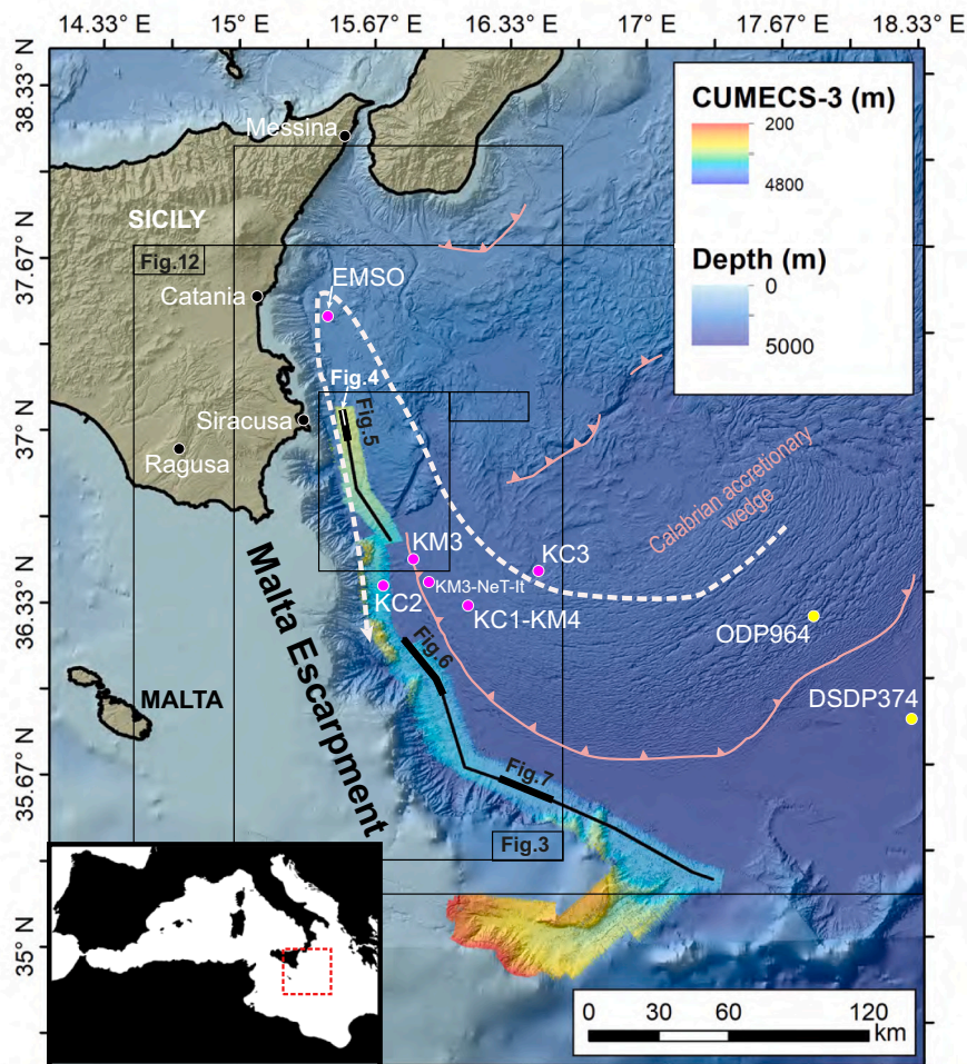
Fig. 1. Location map. Bathymetry base from a compilation of datasets including the compilation published by Gutscher et al. (2017) and CUMECS-3 data. Positions of Fig. 3 and S1 (sediment wave field), sub-bottom (Fig. 4) and seismic profiles (Figs. 5–7), Fig. 12 (average current field), of moorings (see Table 1) and of KM3NeT-It, of DSDP Site 374 and ODP Site 964 are shown.
