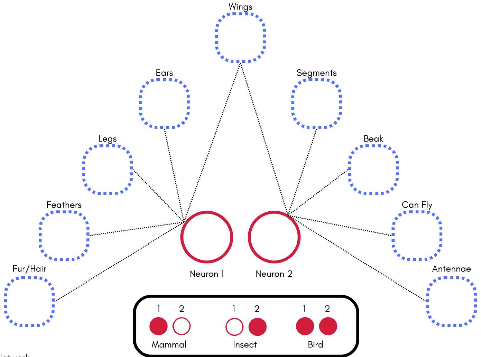
Neural Network
